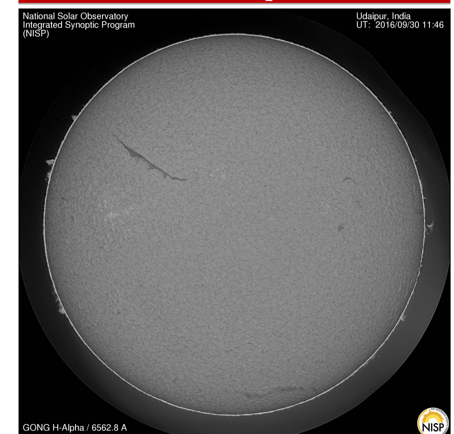
A full disk solar image taken in H-alpha from the GONG instrument on 30 September 2016
