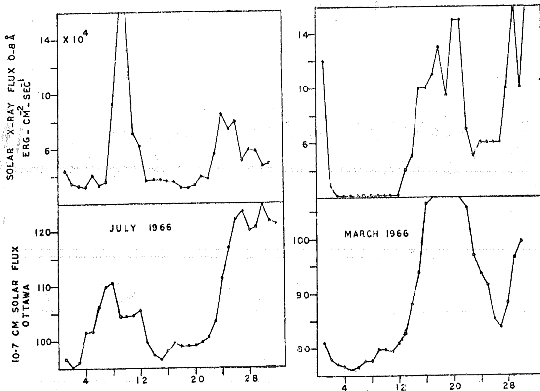
FIG. 7. Intensity of solar X-rays (0-8 Å) and of 10.7 cm. radio-waves in March and July 1966.
