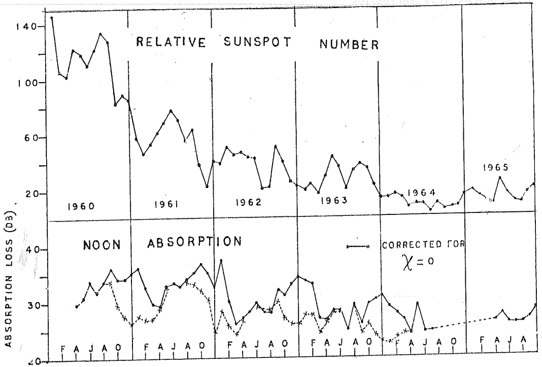
FIG. 3. Variation of monthly noon absorption of 164 kHz radio-waves (1960-65) with sunspot number.
