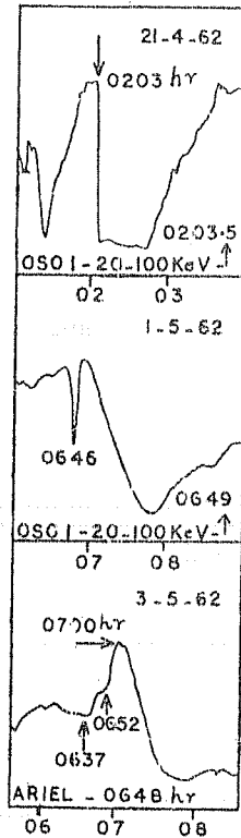
FIG. 4. Signal strengths of Tashkent 164 kHz received at Ahmedabad and solar X-rays from flares, telemetered from OSO 1 and ARIEL satellites.
