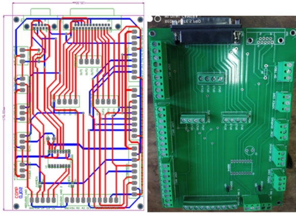
Figure 16. PCB design and PCB board of temperature controller.
