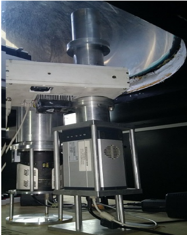
Figure 21. Photograph of CMAP operating from the Optical Aeronomy observatory at PRL's Thalje campus. The filter wheel assembly and the optical dome on the top can be seen clearly.
