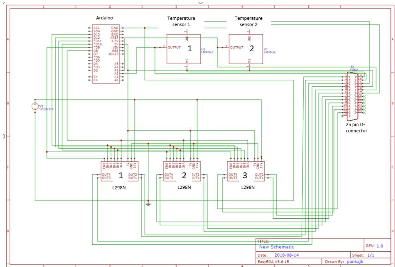
Figure 15. Schematic of temperature controller shows the interfacing between Arduino, bipolar driver (L298N), and temperature sensor (LM35).
