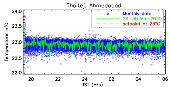
Figure 25. Temperature stability curve for filter wheel chamber with set temperature at 23^{\circ}\text{C} for 30 days of data obtained from Thalje, Ahmedabad in blue color. The highlighted plot shown in green color is for the night of 29 March 2020 obtained from Thalje, Ahmedabad.
