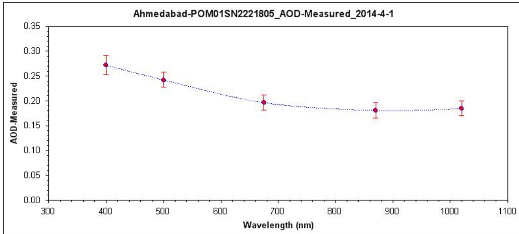
Figure 6. Spectral variation of aerosol optical depth (AOD) over Ahmedabad
