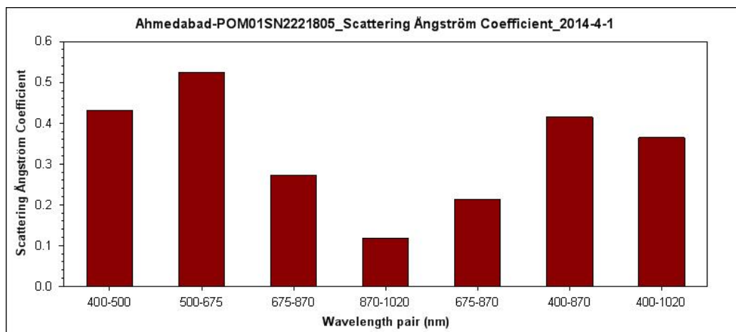
Figure 19. Scattering component of Ångström exponents over Ahmedabad for different wavelength pairs
