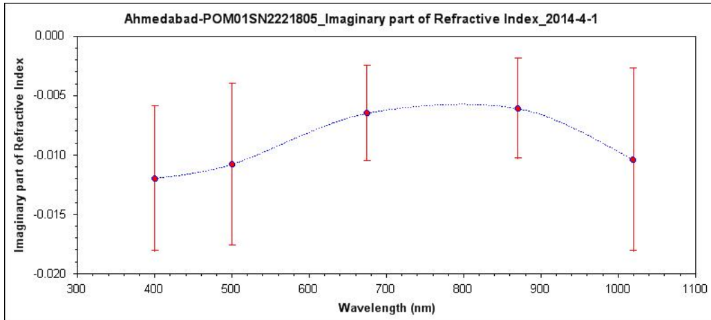
Figure 9. Spectral variation of imaginary part of the refractive index over Ahmedabad
