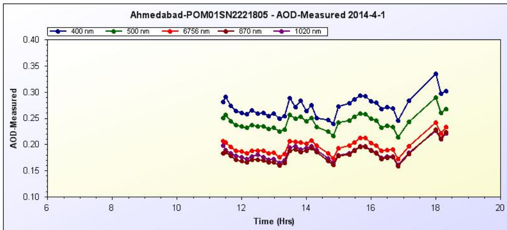
Figure 5. Aerosol optical depth (AOD) variation over Ahmedabad
