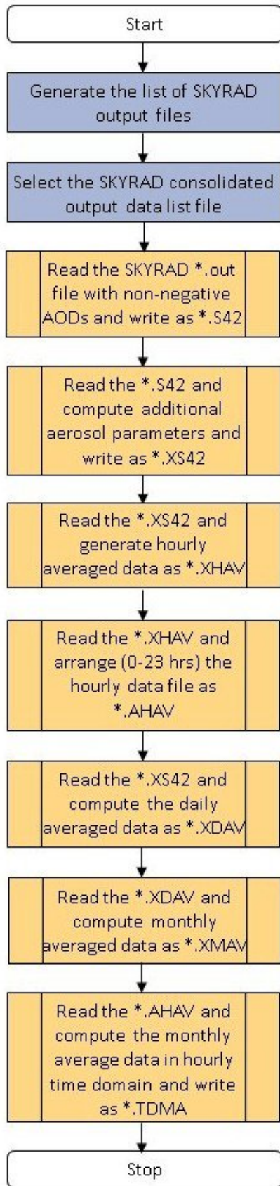
Figure 2. Flowchart of the SKYRAD data analysis and visualization software package
