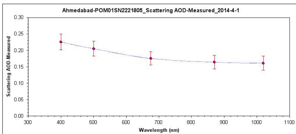
Figure 14. Spectral variation of scattering component of AOD over Ahmedabad
