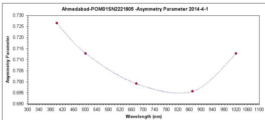
Figure 12. Spectral variation of asymmetry parameter over Ahmedabad
