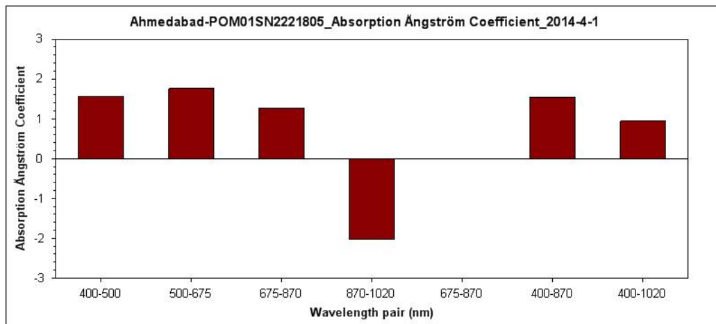
Figure 18. Absorbing component of Ångström exponents over Ahmedabad for different wavelength pairs
