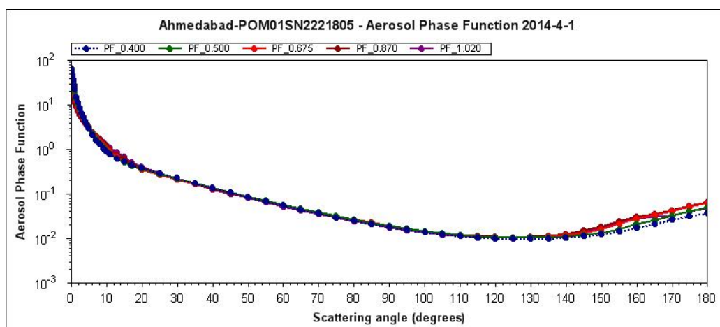
Figure 11. Aerosol phase function for 0 to 180° scattering angles over Ahmedabad
