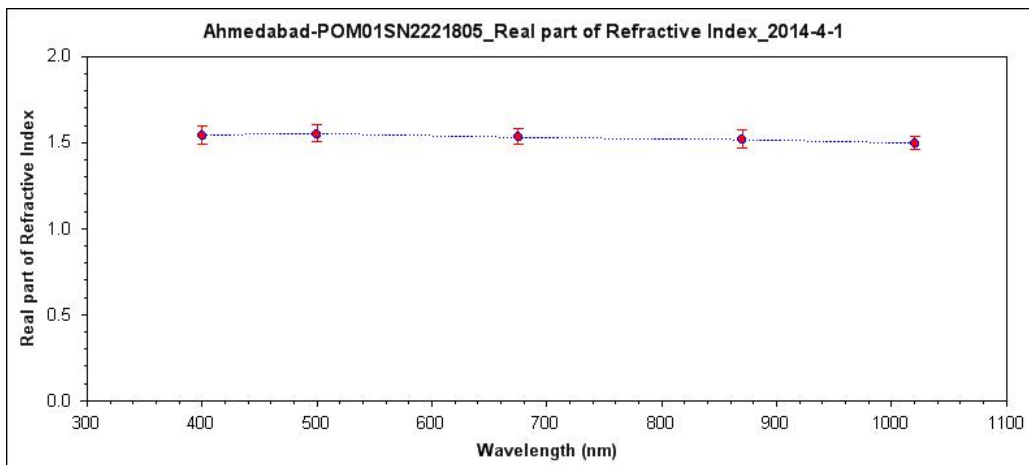
Figure 10. Spectral variation of real part of the refractive index over Ahmedabad
