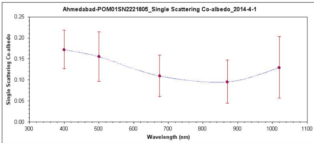
Figure 8. Spectral variation of single scattering co-albedo over Ahmedabad
