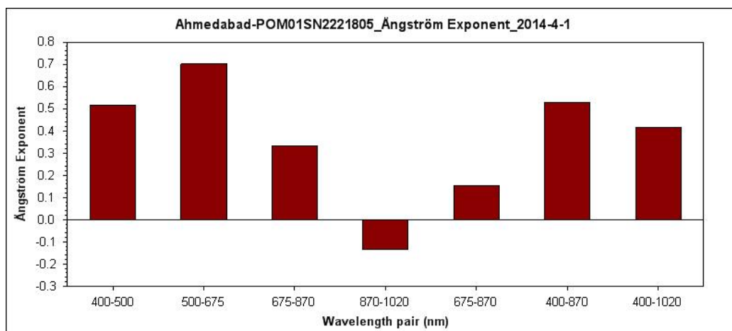
Figure 16. Ångström exponents over Ahmedabad for different wavelength pairs
