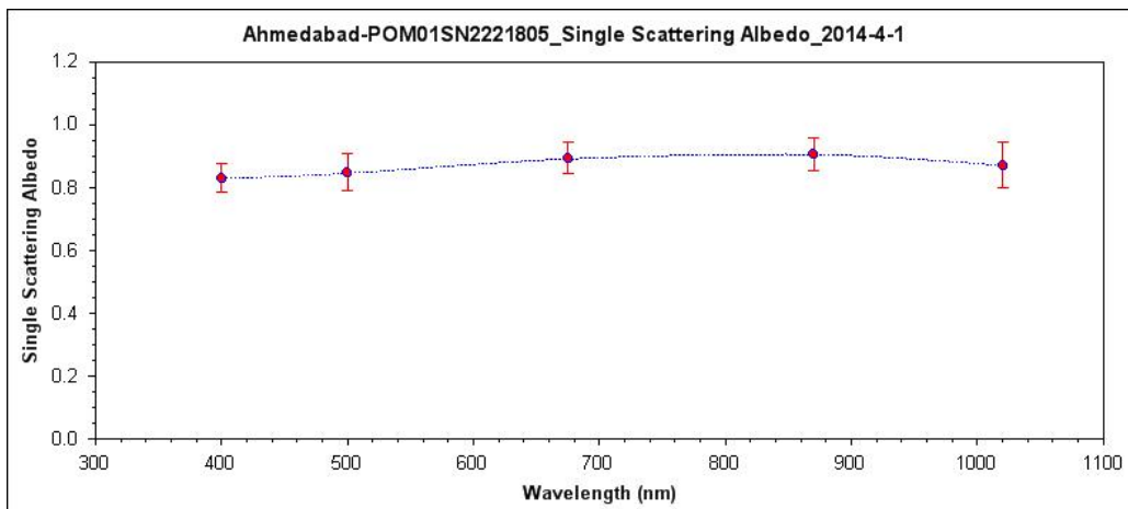
Figure 7. Spectral variation of single scattering albedo (SSA) over Ahmedabad
