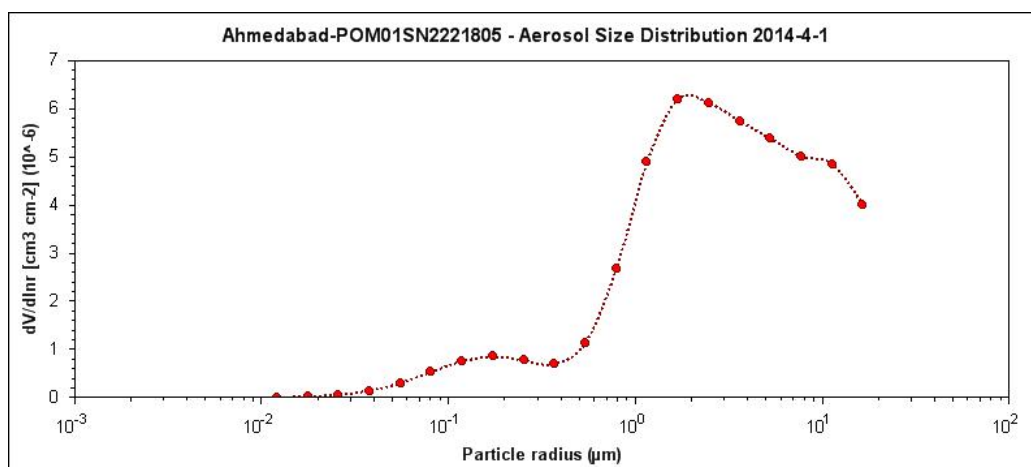
Figure 13. Aerosol volume size distribution over Ahmedabad
