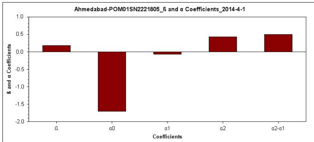
Figure 17. \alpha , \beta , \alpha_1 , \alpha_2 and \alpha_2 - \alpha_1 over Ahmedabad
