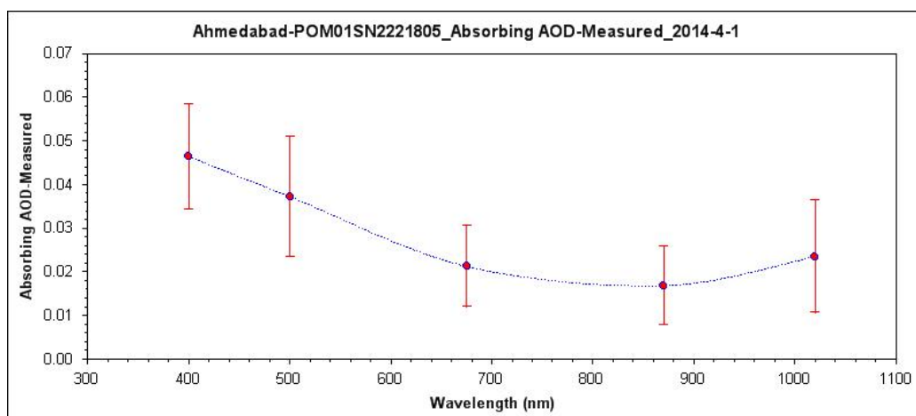
Figure 15. Spectral variation of absorbing component of AOD over Ahmedabad
