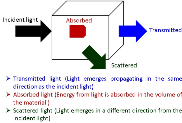
Figure 1. Scattering, absorption and transmission of light
