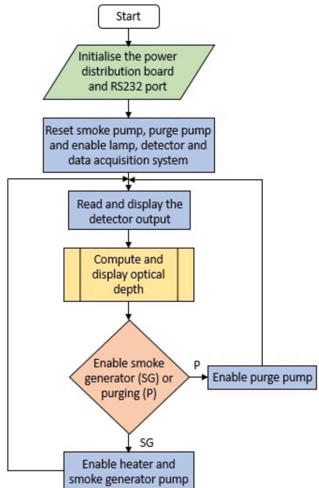
Figure 11. Flowchart for the laboratory simulation of atmospheric transmission
