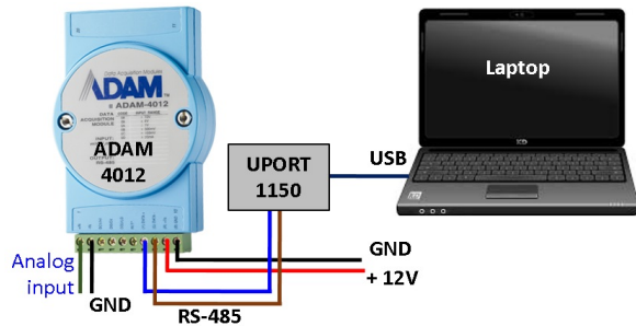
Figure 9. ADAM 4012 and ADAM 4520 based data acquisition system
