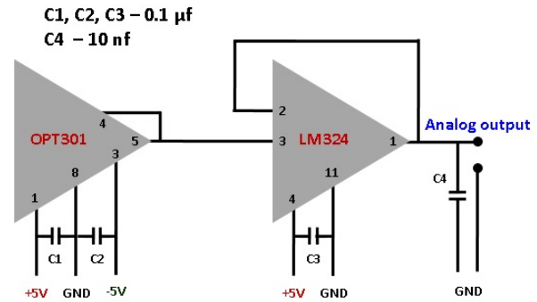
Figure 8. Photodiode signal processing circuit
