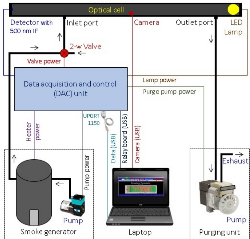
Figure 3. Schematic of the laboratory simulation of atmospheric transmission
