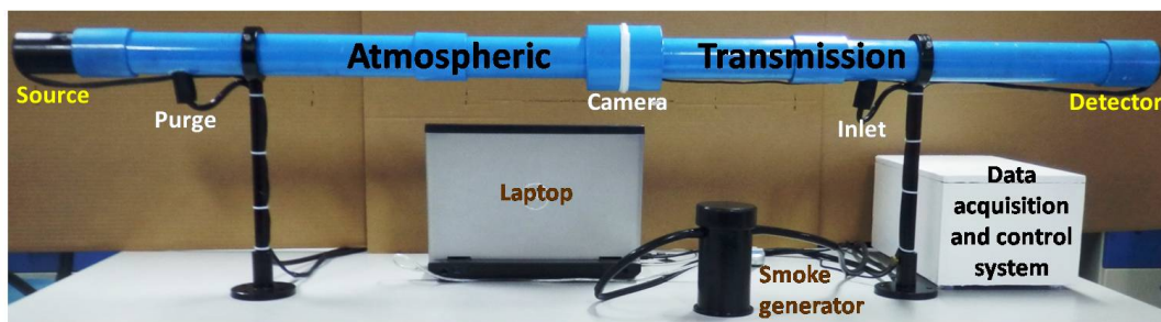
Figure 5. Picture of the laboratory simulation of atmospheric transmission
