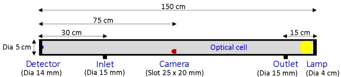
Figure 4. Mechanical schematic of the optical cell
