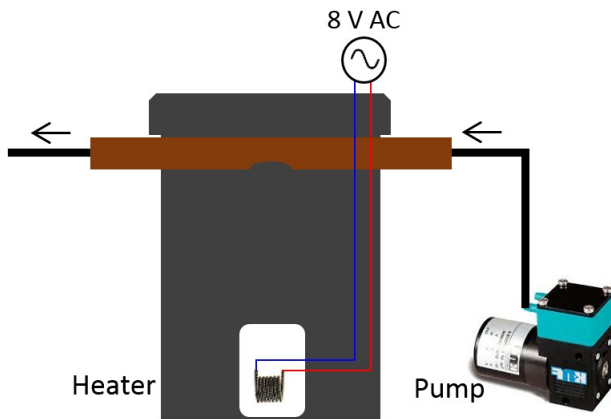
Figure 6. Schematic of the smoke generator used with laboratory simulation of atmospheric transmission
