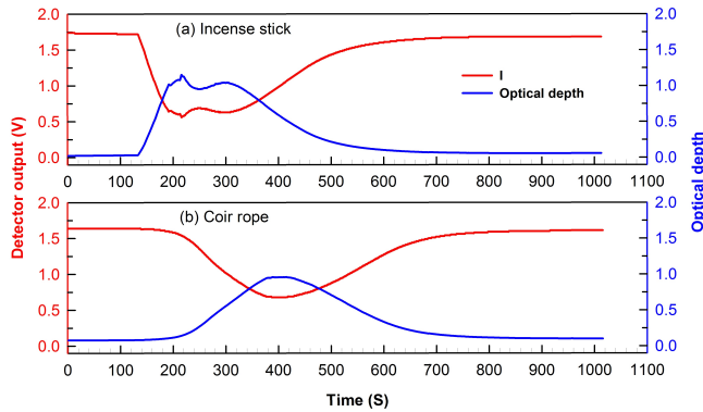
Figure 14. Real time variations of detector light intensity ( I ) and optical depth with incense stick and coir rope burning
