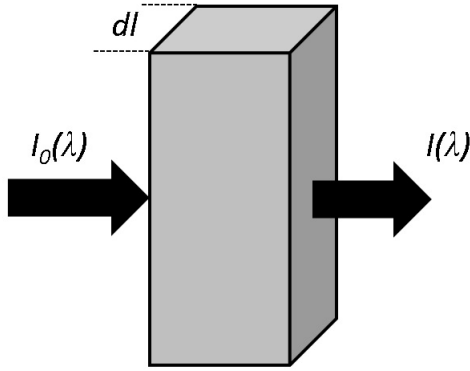
Figure 2. Incident light, I_0(\lambda) passing through an infinitesimally thin layer, dl with ' n ' concentration of particles ( cm^{-3} )
