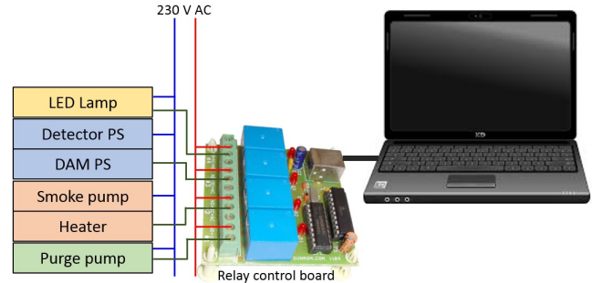
Figure 10. Schematic of the relay control board #1189 interface
