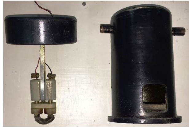
Figure 7. View of the smoke generator used with laboratory simulation of atmospheric transmission
