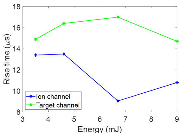
Figure 28. Signal rise time for ion channel and target channel. Read text for further description.
