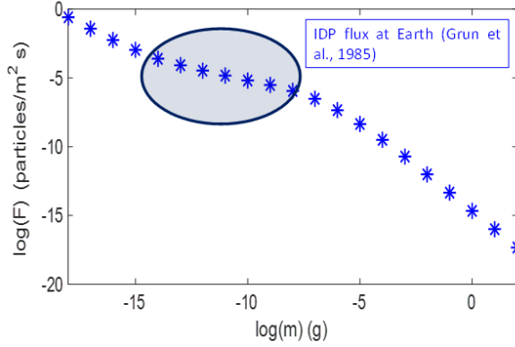
Figure 3. Flux at 1 AU (modified after Grün et al. (1985))
