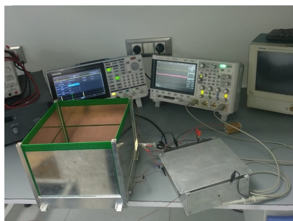
Figure 16. Laboratory test setup where detector and electronics is tested using function generator and oscilloscope
