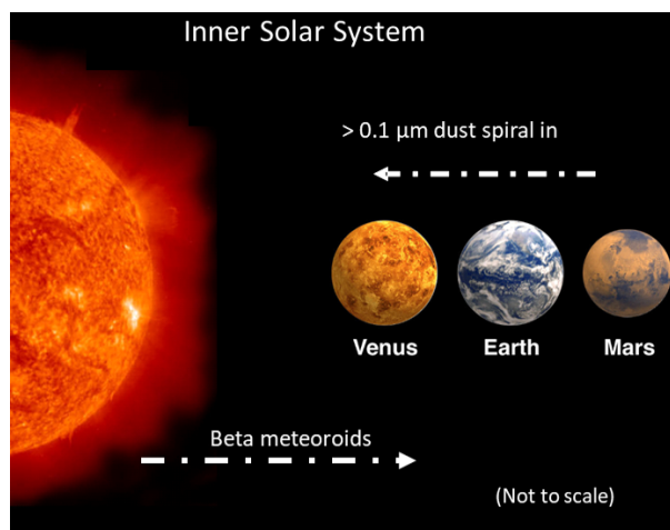
Figure 1. Dynamics of dust within solar system due to different forces. Larger particles spiral inwards because of gravitational force while smaller particles are blown outwards because of radiation pressure.
