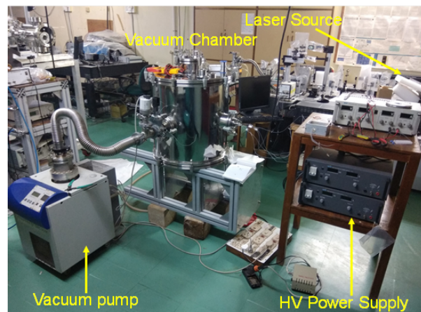
Figure 23. Nanosecond pulse laser test setup at IPR Gandhinagar
