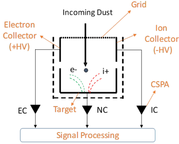
Figure 4. Working principle of dust detector (modified after Pabari et al. (2018))
