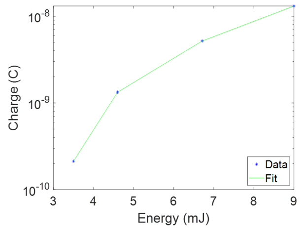
Figure 27. Charge generated during pulse laser experiment with different laser energy and a cubic fit to the data.
