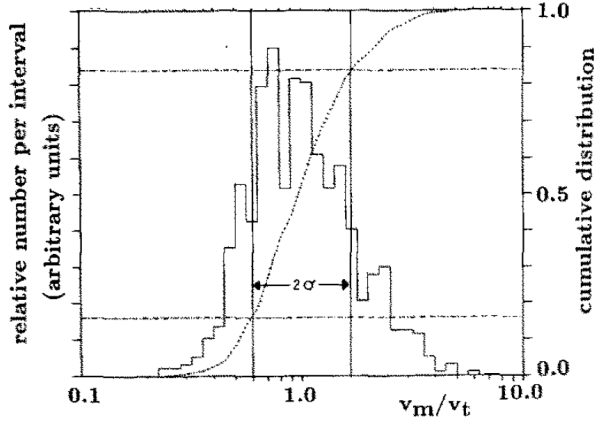
Figure 22. The logarithmic distribution of the ratio of measured velocity to true velocity for Galileo dust detector, taken from Göller and Grün (1989)
