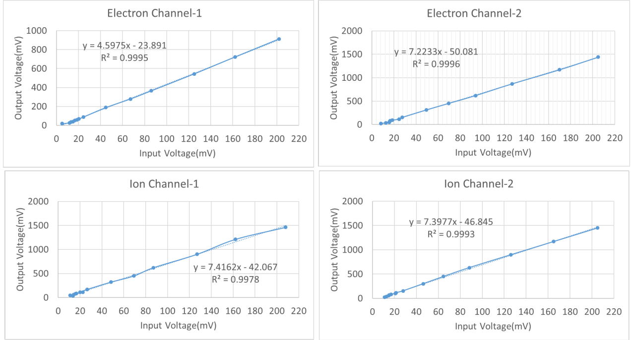
Figure A3. Linearity Test of different buffer configurations for all the collecting plates
