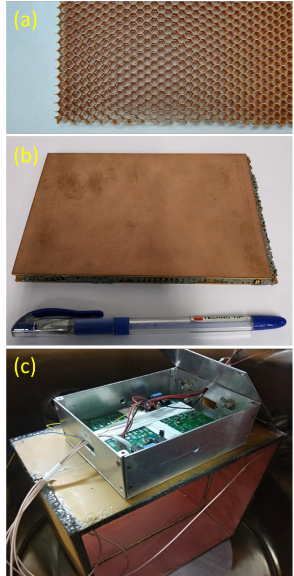
Figure 8. (a) Honeycomb shaped Nomex sheet (b) Composite structure fabricated using Nomex as core and Copper coated PCB as face (c) Detector fabricated using commercial Nomex
