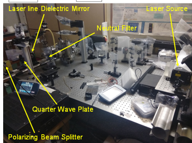
Figure 24. Diagram showing optical setup at IPR. The laser beam is passed through polariser and beam splitter and eventually focused using lens on the detector lying inside the vacuum chamber.
