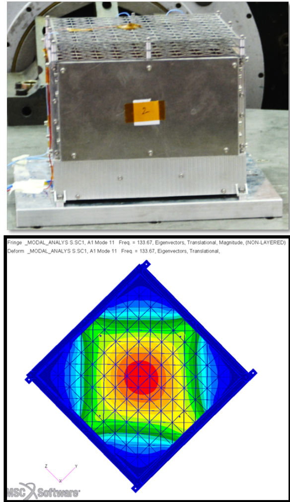
Figure 19. Top pane: Dust detector model on vibration shaker. Bottom pane: Vibration analysis result shows the fundamental mode of 134 Hz in Z-direction.
