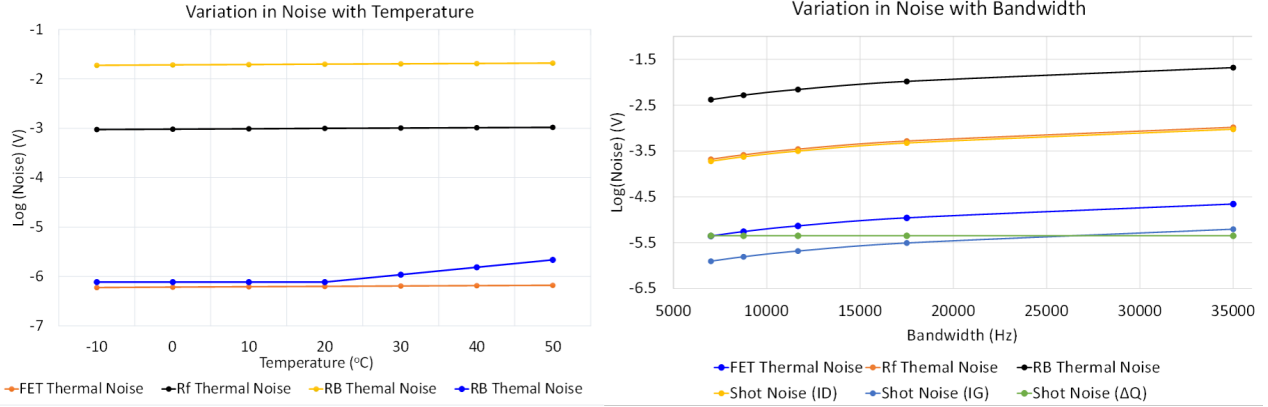
Figure A2. Variation in noise from different sources due to Temperature (left) and bandwidth (right). As observed thermal noise from resistors contributes the most.
