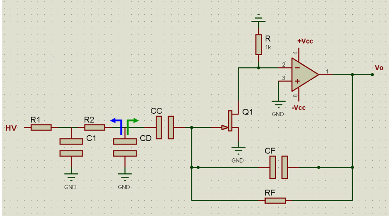
Figure A1. Analog circuit with different noise generating sources discussed in the section. The arrow above detector capacitor CD shows the two path for current of which blue colored one is high impedance path and green color shows low impedance path.
