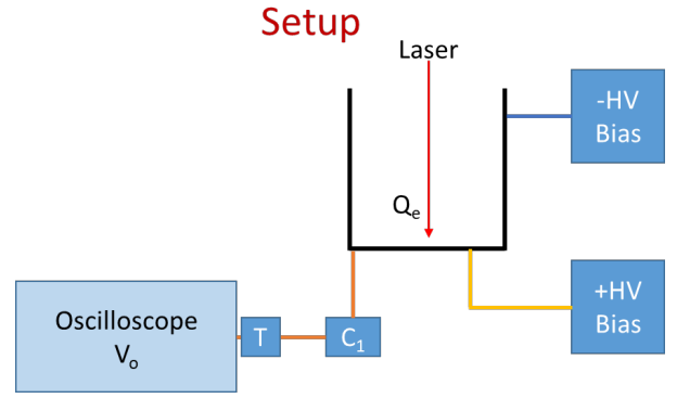
Figure 26. Test setup at IPR to derive the equivalence relation
