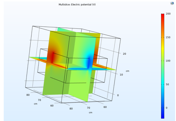
Figure 7. Electric potential slice plot for the detector geometry modelled in COMSOL software
