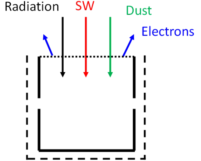
Figure 14. Components that the dust detector will encounter in space
