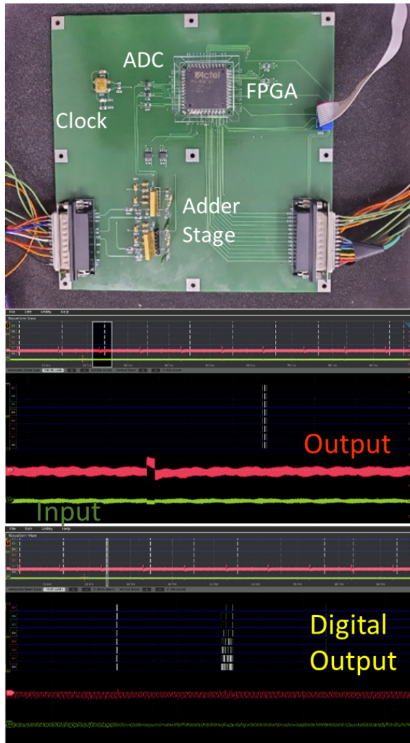
Figure 18. Top pane: Processing electronics card of dust detector. Mid pane: The input to detector and output of front end electronics. bottom pane: Data frame generated by FPGA are shown.
