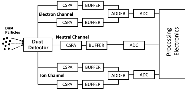
Figure 9. Electronics schema of VODEX
