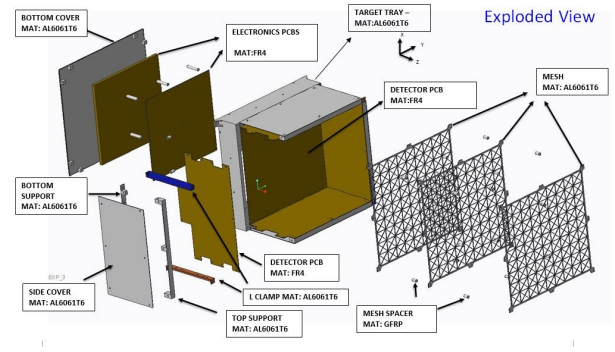
Figure 6. Exploded view of Dust Detector
