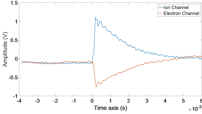
Figure 25. A typical output from pulse laser test of dust detector
