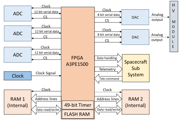
Figure 11. Processing electronics of VODEX
