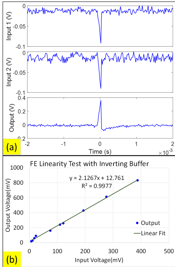
Figure 17. Linearity test of Detector + CSPA + Buffer configuration
