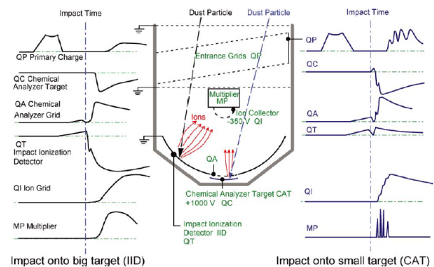
Figure 20. Detection principle and signal measurements carried out by Cosmic Dust Analyser which was flown on-board Cassini, taken from Srama et al. (2004)
