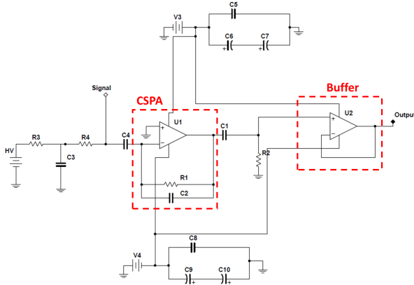
Figure 10. CSPA and Buffer configuration
