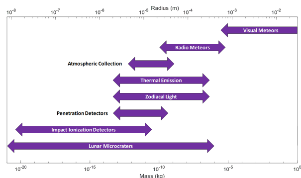
Figure 2. Different detection techniques to study IDPs in different mass or size ranges (modified after Sykes et al. (2004)). Larger particles are observed visually or through radio echo from ionizing meteoroids. Atmospheric collections of an IDP's remaining are usually carried out using aeroplanes. Large scale survey of micron sized particles are carried out using zodiacal light or infrared observations. To study smaller particles in-situ detectors are used while lunar microcrater study allows analysis of larger range of particle size, however, this requires lunar sample.
