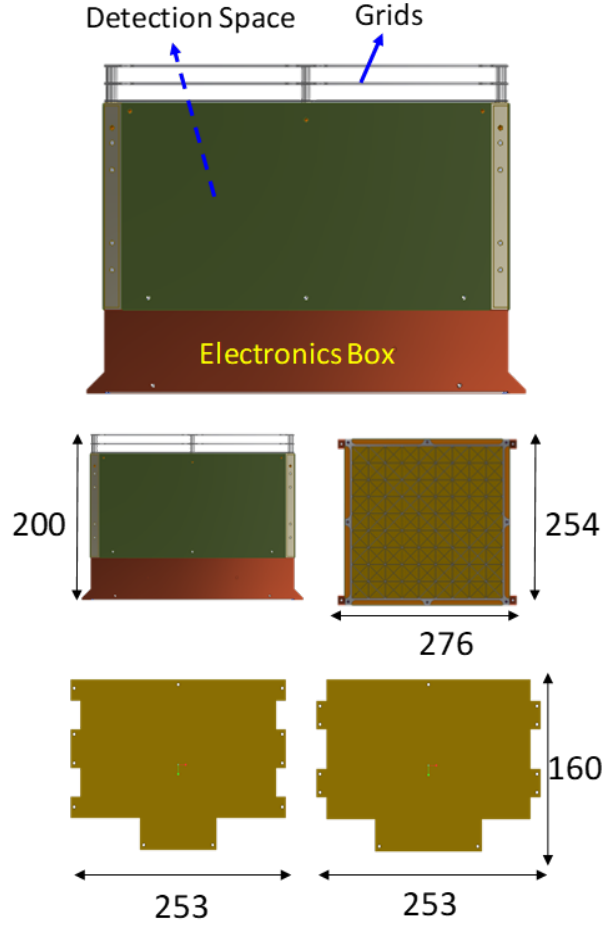
Figure 5. Mechanical Design of VODEX with overall dimensions and dimensions of detector PCBs. All dimensions are in mm.
