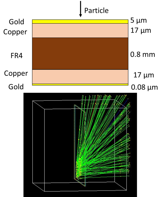
Figure 15. Top pane: The structure of target material with thickness of each layer. Bottom pane: A snapshot of simulation run with target material at centre in GEANT4 software. The green lines show trajectory of impacting particles at different angles.
