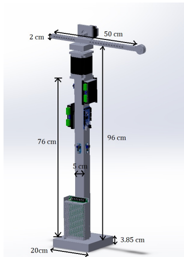
Figure 3. Drawing of the Automated Freeze-Thaw mechanism using the CAD software Solidworks
