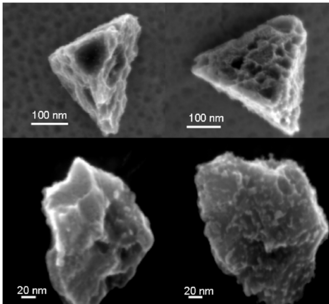
Figure 1. Secondary Electron (S.E.) images of Presolar Silicon Carbide (SiC) grains isolated from meteorites by Chemical Separation method. Irregular grain surfaces are the result of chemical etching
