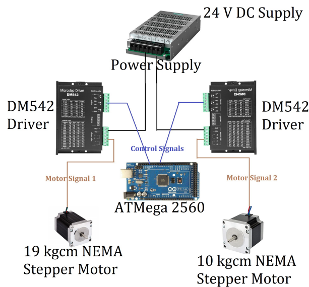
Figure 4. Schematic diagram representing the electronic controls of motors, including the three main components: power supply, motor drivers and the microcontroller
