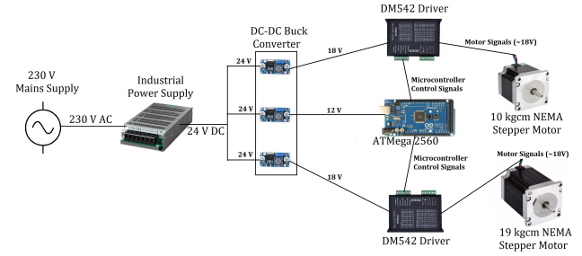
Figure 6. The schematic diagram showing the power distribution for the Automated Freeze-Thaw instrument
