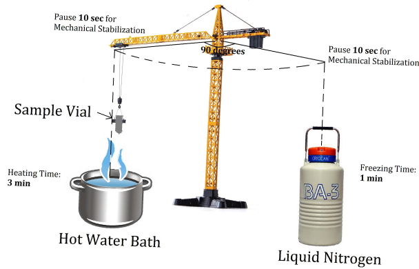
Figure 2. Schematic diagram of the algorithm of operation of the Automated Freeze-Thaw (AFT) instrument including the major elements
