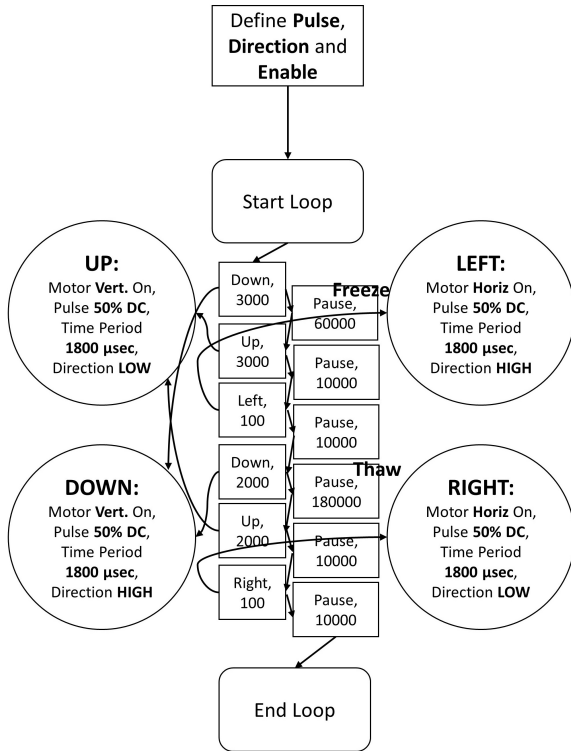
Figure 5. Programming Logic for Motor control
