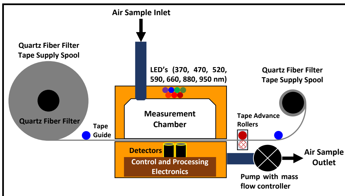
Figure 1. Schematic of aethalometer
