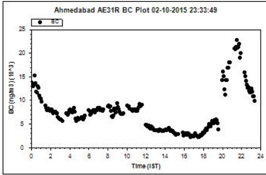
Figure 7. Averaged BC diurnal plot for October 02, 2015 at Ahmedabad
