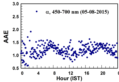
Figure 12. Diurnal variation of Ångström absorption exponent (AAE) for the wavelength pair 450-700 nm over Ahmedabad on August 08, 2015
