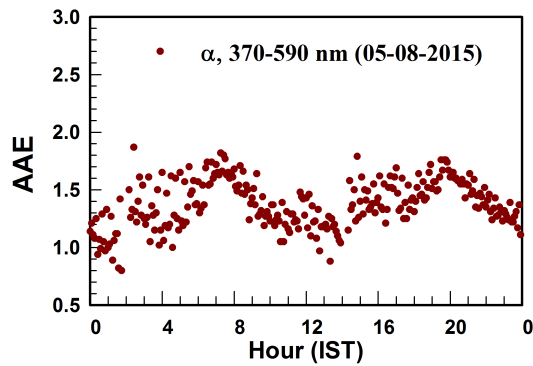
Figure 11. Diurnal variation of Ångström absorption exponent (AAE) for the wavelength pair 370-590 nm over Ahmedabad on August 08, 2015
