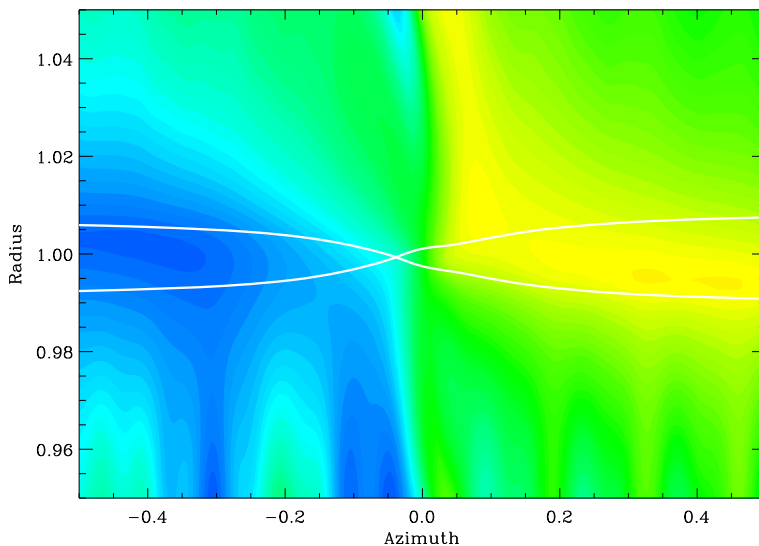
Fig. 6.5 Perturbed surface density in the coorbital region of an Earth-mass planet in a disc with h = 0.05 and \alpha = 0 (uniform background surface density). The planet is located at r = 1 , \varphi = 0 . The solid curves show the separatrices of the planet's horseshoe region. In order to remove the planet's wakes and to render this map more legible, we have subtracted the density perturbation obtained in a situation where no corotation torque is expected (namely \alpha = 3/2 , as will be shown below). This cancellation is imperfect, however, as the wakes of the two cases are not strictly identical
