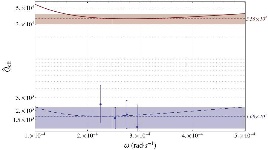
Fig. 7.20 Dependence to the perturbative strain pulsation \omega of the tidal quality factor \hat{Q}_{\text{eff}} Jupiter-like (red solid line) and Saturn-like (blue dashed line) giant planets. Note that the curves are represented with a logarithmic scale. The red and blue dotted lines correspond to the mean value of \hat{Q}_{\text{eff}} = \{(3.56 \pm 0.56) \times 10^4, (1.682 \pm 0.540) \times 10^3\} (for Jupiter and Saturn respectively) determined by Lainey et al. [60, 61]. Their zone of uncertainty is also represented in the corresponding color. The blue dots correspond to the values (obtained by Lainey et al. [61]) of the dissipation induced in Saturn by Enceladus, Thetys, Dione and Rhea with their respective error bars. We recall the values of R_p = \{10.97, 9.14\} (in units of R_p^\phi , the Earth radius), M_p = \{317.8, 95.16\} (in units of M_p^\phi , the Earth mass), M_c = \{6.41, 18.65\} \times M_p^\phi , and R_c = \{0.15, 0.26\} R_p . We take for the viscoelastic parameters G = \{2.73, 6.51\} \times 10^{10} (Pa), and \eta = \{8.65 \times 10^{13}, 2.50 \times 10^{14}\} (Pa · s) for Jupiter and Saturn respectively. (Adapted from Remus et al. [93]; courtesy Astronomy & Astrophysics)
