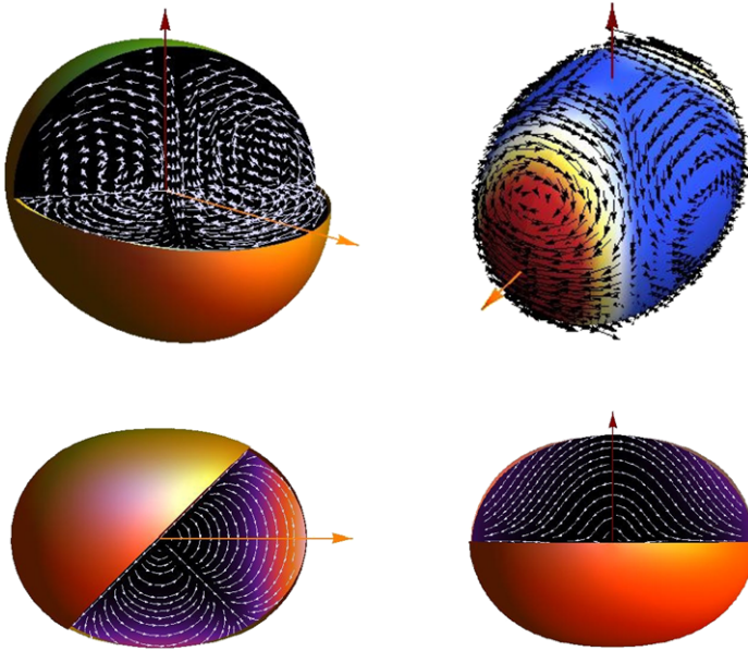
Fig. 7.11 Top-left : 3-D view of the total (poloidal and toroidal) adiabatic equilibrium tide velocity field (white arrows). The red and orange arrows indicate the direction of the primary's rotation axis and the line of centers respectively. Top-right : Representation of this velocity field at the surface of the primary (black arrows); the color-scaled background represents the normalised tidal potential intensity (blue and red for the minimum and maximum values respectively). Bottom-left : View of the velocity field (white arrows) in its equatorial plane of symmetry; the color-scaled background represents the velocity value (black and orange for the minimum and maximum values respectively). Bottom-right : View of the velocity field (white arrows) in its meridional plane of symmetry; the color-scaled background represents the velocity value (black and purple) for the minimum and maximum values respectively. (Taken from Remus et al. [94], courtesy Astronomy & Astrophysics)
