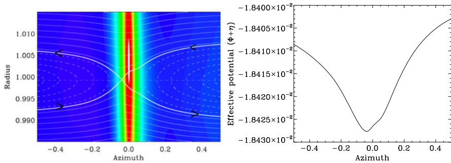
Fig. 6.3 Left: streamlines in the vicinity of an Earth-mass planet embedded in a disc with H/r = 0.05 . The softening length of the potential is \varepsilon = 0.6H . The thick lines show the separatrices of the horseshoe region (the frontiers between the dashed streamlines that exhibit horseshoe-like motion and the solid ones corresponding to circulating material with respect to the planet orbit). A few arrows show the flow's direction with respect to the planet. The horizontal dashed line shows the corotation radius, where the angular velocities of the disc and the planet are equal. Right: effective potential at the corotation radius, as a function of azimuth
