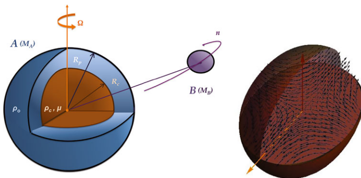
Fig. 7.18 Left: Two-layer model of planetary internal structure (body A of mass M_A rotating at angular velocity \Omega ) formed by an internal rocky core surrounded by a fluid envelope perturbed by a companion (body B of mass M_B orbiting around A with mean motion n ). R_c and R_p are respectively the core and the planetary radii, \rho_o and \rho_c the densities of the fluid envelope and of the core, and \mu is the shear modulus of the core. Right: purely elastic tidal displacement in the solid core free of fluid envelope; the red and orange arrows indicate respectively the symmetry axis of the planetary core and the direction of the companion. (Taken from Remus et al. [93]; courtesy Astronomy & Astrophysics)
