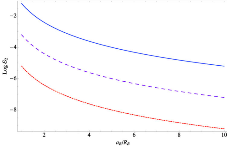
Fig. 7.5 \text{Log } \mathcal{E}_2 in function of a_B/R_B for J_2 = 10^{-3} (red dashed line), 10^{-2} (purple long-dashed line), 10^{-1} (blue solid line). The non-punctual terms have to be taken into account for strongly deformed perturbers ( J_2 \geq 10^{-2} ) in very close systems ( a_B/R_B \leq 5 ) while they decrease rapidly otherwise. (Taken from Mathis and Le Poncin-Lafitte [77], courtesy Astronomy & Astrophysics)
