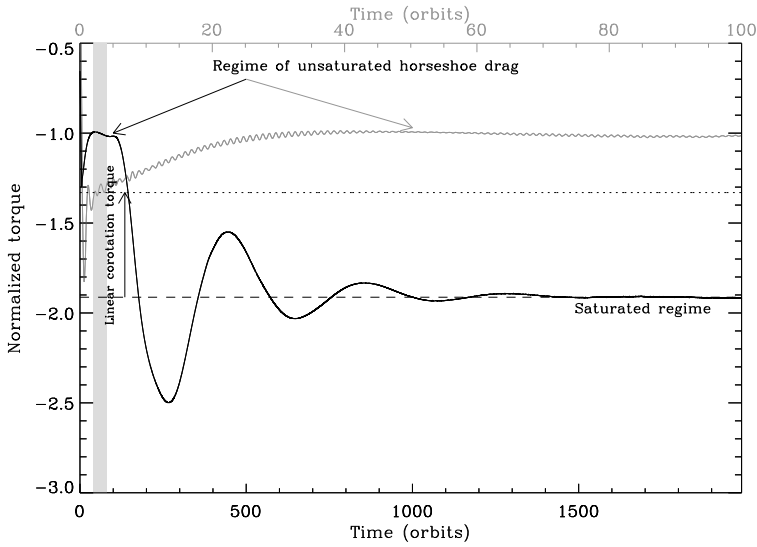
Fig. 6.4 Time evolution of the total torque (sum of the differential Lindblad torque and corotation torque) on a M_p = 10^{-6} M_\star planet mass embedded in an inviscid isothermal disc. The black curve (bottom x-axis ) shows the torque evolution over 2000 planet orbits, while the grey curve (top x-axis ) focuses on the evolution over the first 100 planet orbits. The dashed line shows the value of the differential Lindblad torque, and the dotted curve highlights the corotation torque predicted with a linear analysis. Taken from [68]
