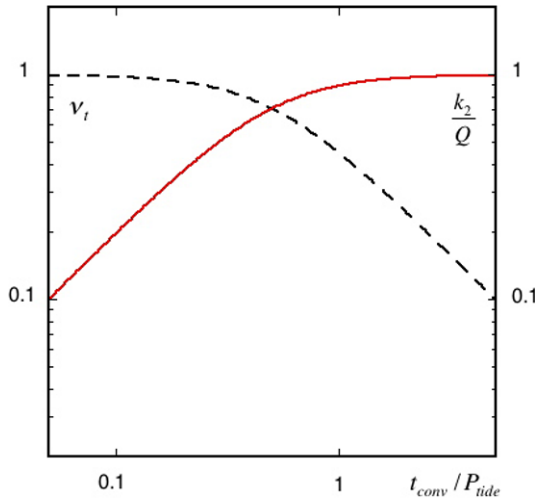
Fig. 8.4 The two regimes of turbulent dissipation (Eq. (8.24)). As long as the local convective turn-over time remains shorter than the tidal period ( t_{\text{conv}} < P_{\text{tide}} ), the turbulent viscosity \nu_t (in black dashed line) is independent of the tidal frequency, and the inverse quality factor k_2/Q (in red continuous line) varies proportionally to the tidal frequency ( \sigma_t ) (so does also the tidal lag angle). When t_{\text{conv}} > P_{\text{tide}} , \nu_t varies proportionally to the tidal period, whereas k_2/Q does no longer depend on the tidal frequency. \nu_t and k_2/Q have been scaled by the value they take respectively for t_{\text{conv}}/P_{\text{tide}} \rightarrow 0 and \rightarrow \infty (from Remus et al. [32], courtesy A&A)
