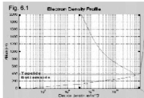
Fig. 5. TEC profile (adapted from the literature)
