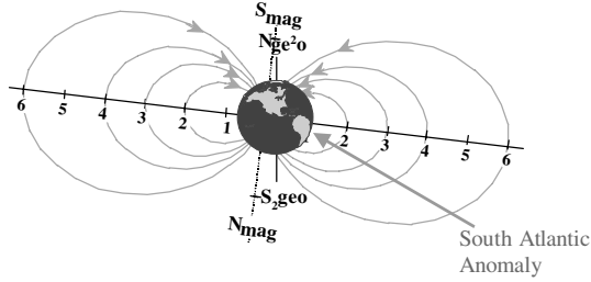
Fig. 3. Dipolar magnetic field tilted and off-center with respect to Earth
