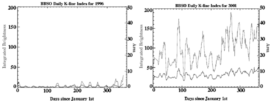
Fig. 15. Big Bear Solar Observatory (BBSO) daily CaII K index. The left panel shows a period of low solar activity (1996) and the right panel a period of strong solar activity (2001) ( http://www.bbso.njit.edu/Research/Cak/ ). The upper index in each panel is the integrated brightness above 7.5% of the central disk brightness; the bottom index is the corresponding area
