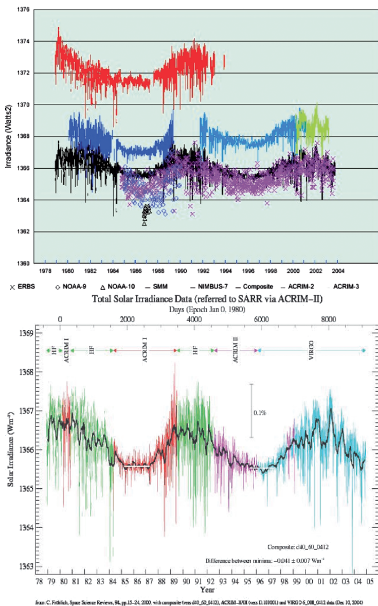
Fig. 3. Various Total Solar Irradiance (TSI) time series measured from space are presented on the upper panel. The composite TSI as daily values plotted in different colors for the different originating experiments is shown on the lower panel (from Fröhlich [8])
