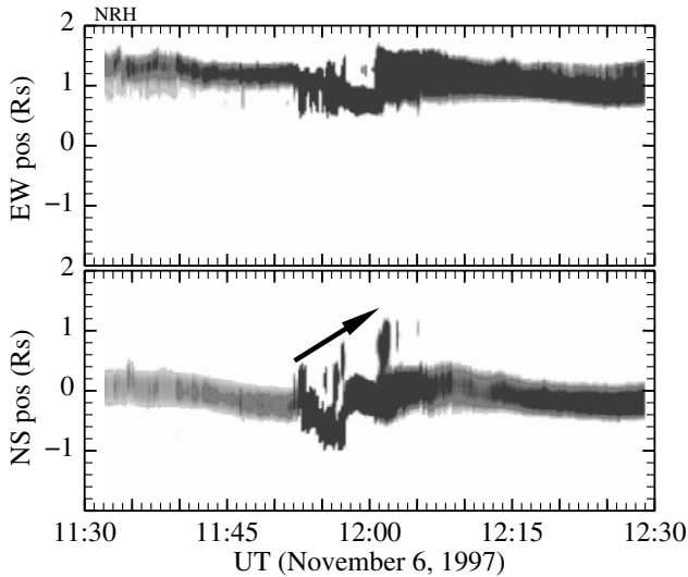
Fig. 17. November 6, 1997: two one-dimensional plots along east–west top and north–south bottom directions showing the space-time evolution of the event at 164 MHz (from [37])
