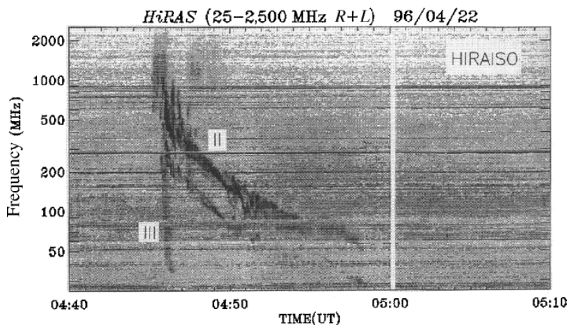
Fig. 6. Dynamical spectrum of April 22, 1996, event from Hiraíso Terrestrial Research Center: type III and type II bursts emitted in the corona (after [21])
