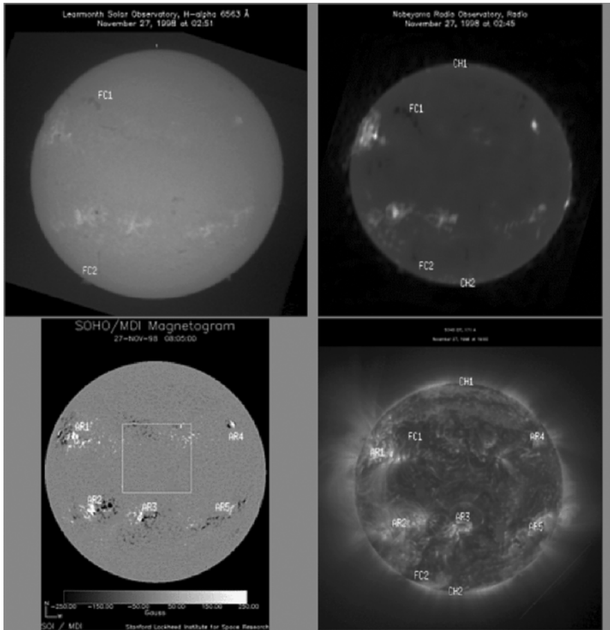
Fig. 1. Multiwavelength observations are useful to determine the nature of the observed structure. Top left: H\alpha disk image; top right: Radio observations; bottom left: Magnetogram; bottom right: EUV coronal image. Example of structures discriminations which appear dark on SOHO/EIT images: Filament Channel -FC- and Coronal Holes -CH- [4, 5]. Coronal Holes are the source of one type of perturbations of the magnetosphere
