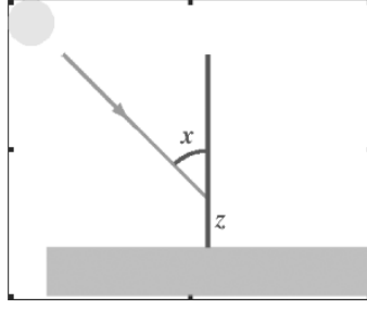
Fig. 22. Propagation of an electromagnetic beam in the atmosphere of an “artificial” flat plane planet (from [42])
