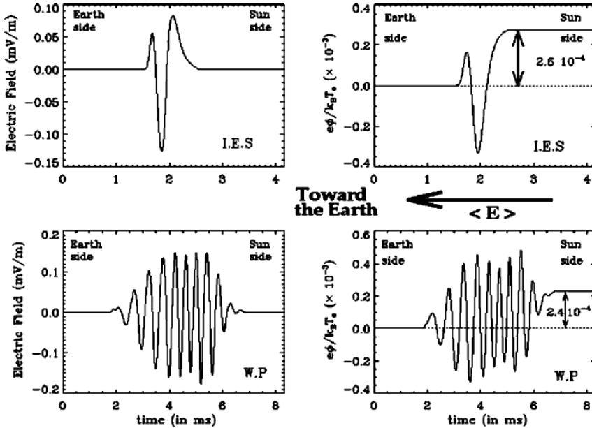
Fig. 13. Example of double layers and wave packet structures measured in the solar wind by WIND. From [45]
