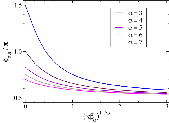
Fig. 4.2 Outer reflection phase \phi_{\text{out}} for attractive inverse-power potentials (4.57) as function of the reduced classical turning point \kappa r_{\text{out}} = (\kappa \beta_\alpha)^{1-2/\alpha} . (Adapted from [85])
