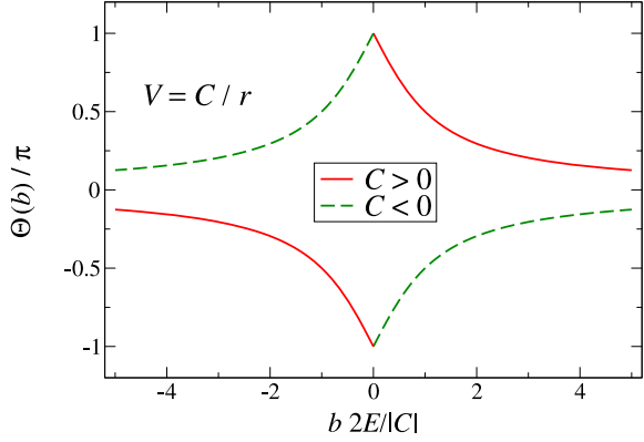
Fig. 1.16 Deflection function (1.24) for the Kepler–Coulomb potential, adapted to the two-dimensional case
