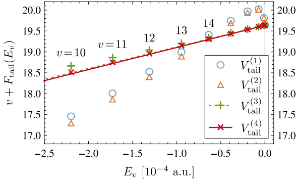
Fig. 4.6 Plots of v + F_{\text{tail}}(E_v) against E_v with the quantization function F_{\text{tail}}(E) defined via (4.16), (4.17) on the basis of the definitions (4.73)–(4.76) of V_{\text{tail}} . The straight dashed green and solid red lines are fitted according to (4.20) through the highest two states, v = 18 and v = 19 , with F_{\text{tail}}(E) based on V_{\text{tail}}^{(3)} and V_{\text{tail}}^{(4)} , respectively. (Adapted from [50])
