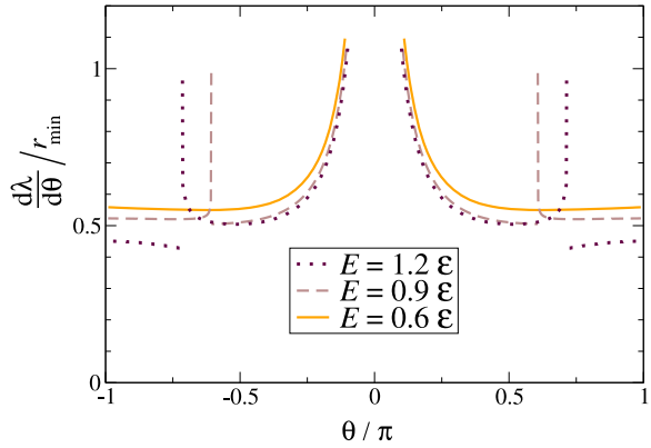
Fig. 1.18 Differential scattering cross section in two dimensions for the Lennard–Jones potential (1.32). For E = 0.9\mathcal{E} , there are rainbows at |\theta| = \theta_R \approx 0.61\pi and the dark sides are towards smaller values of |\theta| . For E = 1.2\mathcal{E} , there are rainbows at |\theta| = \theta_R \approx 0.71\pi and the dark sides are towards larger values of |\theta|
