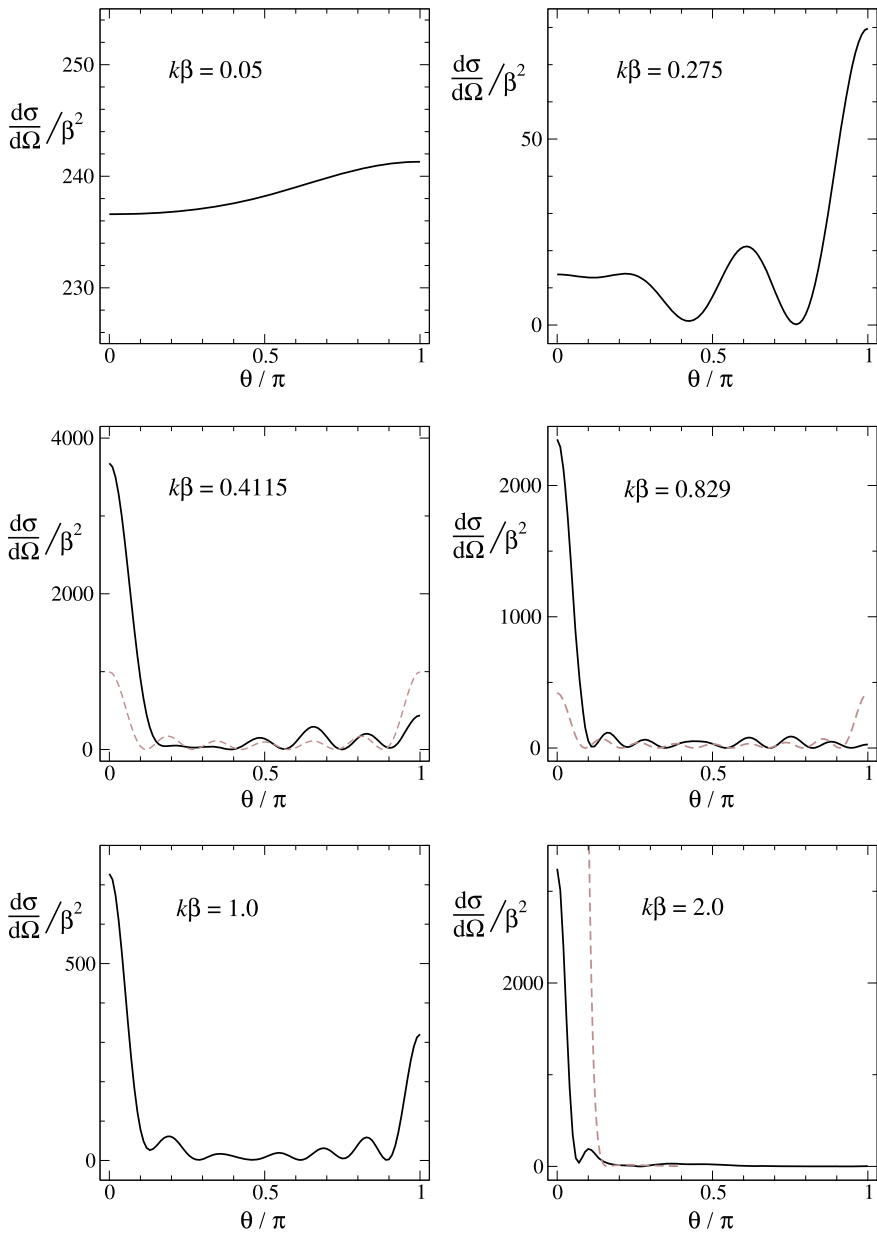
Fig. 2.13 Angular distributions for the differential cross sections for scattering by the model potential (2.105). The dashed lines at k\beta = 0.4115 and k\beta = 0.829 show the function (2l+1)^2 P_l(\cos\theta)^2 / k^2 for l=6 and l=8 , respectively. The dashed line at k\beta = 2.0 shows the result of the Born approximation (2.135)
