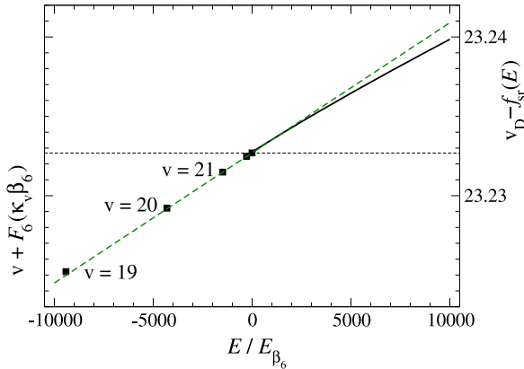
Fig. 4.12 For the Lennard–Jones potential (4.68) with B_{\text{LJ}} = 10^4 , the left-hand part ( E < 0 ) shows v + F_6(\kappa_v \beta_6) as function of energy for the highest five bound states v = 19, \dots, 23 (solid squares). The right-hand part ( E > 0 ) shows v_D - f_{\text{sr}}(E) , derived from the exact numerically calculated phase shifts by resolving Eq. (4.119). The dashed horizontal line indicates the value v_D = 23.2327 of the threshold quantum number; the other dashed line shows the linear function v_D - \gamma_{\text{sr}}E , with \gamma_{\text{sr}} = -1.16/\mathcal{E} = -8.2 \times 10^{-7}/E_{\beta_6} , compare Table 4.5
