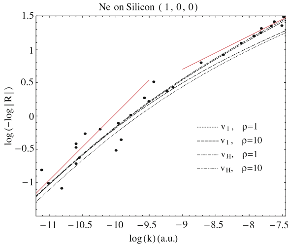
Fig. 4.9 Modulus of the quantum reflection amplitude, as observed in the scattering of metastable neon atoms off a silicon surface [78]. The figure shows \ln(-\ln |R|) as function of \ln(k) (natural logarithms) with k measured in atomic units, i.e. in units of the inverse Bohr radius. The curves show the results obtained by numerically solving the Schrödinger equation (4.11) with potentials (4.99) constructed with the shape functions v_1 and v_H . The quantum length \beta_4 associated with the strength C_4 of the potential in the highly retarded limit is \beta_4 = 11400 a.u. in all cases. For the -C_3/r^3 van der Waals limit of the potential, the quantum length is \beta_3 = 11400 a.u. for \rho = 1 and \beta_3 = 114000 a.u. for \rho = 10 . The straight red line in the bottom left corner shows the behaviour \ln |R| \sim -2\beta_4 k expected in the low- k regime. The straight red line in the top right corner shows the behaviour \ln |R| \propto -\sqrt{\beta_4 k} expected in the high- k regime for a single-power 1/r^4 potential. (From [33])
