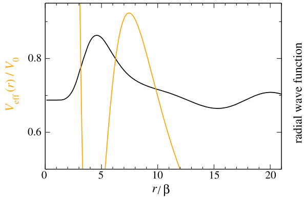
Fig. 2.10 Solution of the radial Schrödinger equation (2.35) with the model potential (2.105) in the partial wave l = 8 at energy E = E_R = 0.6872V_0 . The orange line shows the effective potential (2.36)
