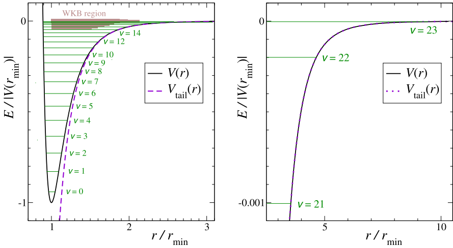
Fig. 4.1 Deep potential falling off faster than 1/r^2 at large distances. The example is actually the Lennard–Jones potential (2.298) with B_{\text{LJ}} = 10^4 , which supports 24 bound states, v = 0, 1, 2, \dots, 23 . The brown shaded area in the left-hand panel schematically indicates where the WKB approximation is accurate at near-threshold energies
