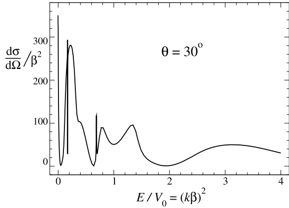
Fig. 2.12 Differential scattering cross section for the model potential (2.105) as function of energy for \theta = 30^\circ
