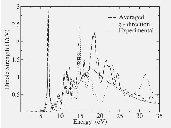
Fig. 4.2. Optical absorption of the benzene molecule. Experimental results from [40]. Figure reproduced from [41]
