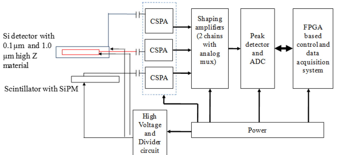
Fig. 15. Block diagram of the electronics for the species separated spectra unit.
