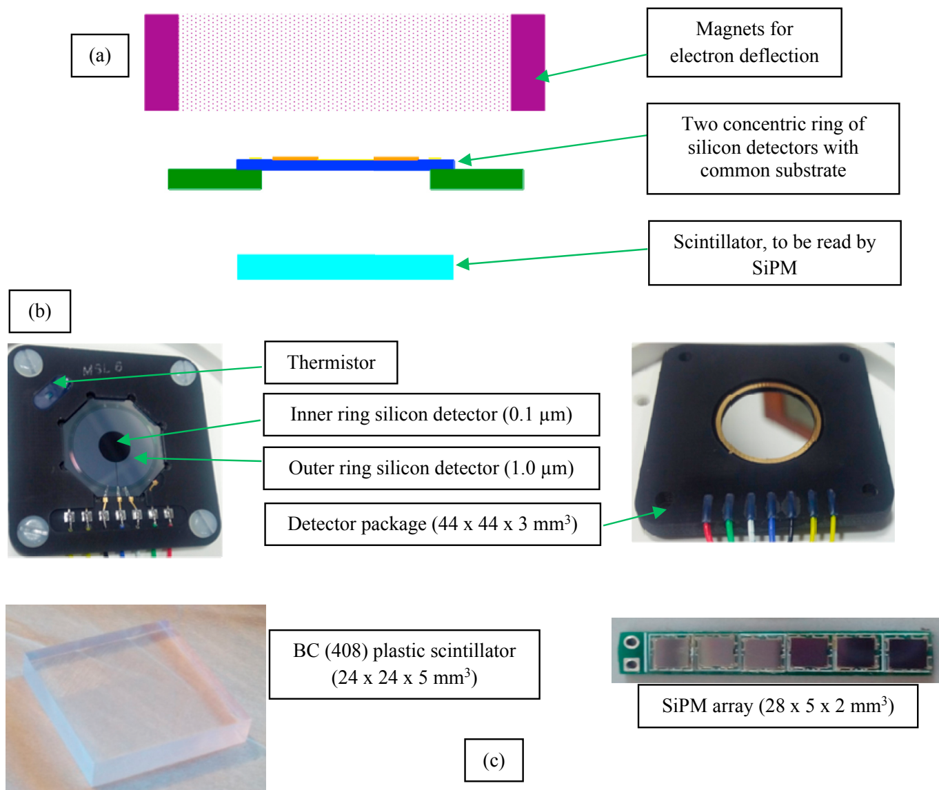
Fig. 9. (a) Detector configuration for particle identification, (b) dual window Si-PIN detector – top view & rear view, (c) plastic scintillator & SiPM array.
