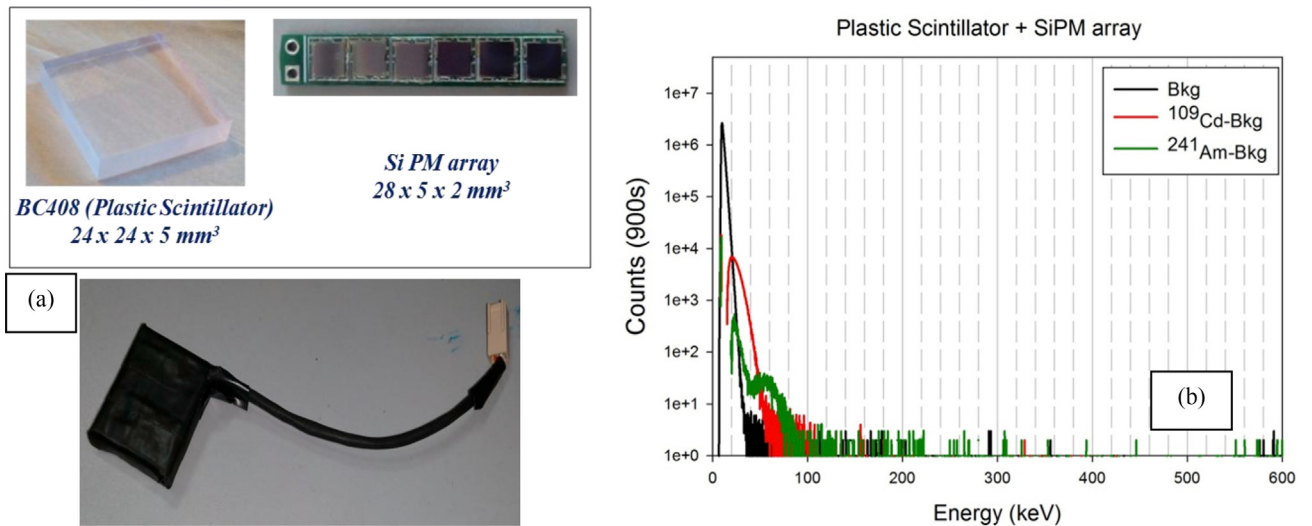
Fig. 17. (a) Plastic scintillator and SiPM array, (b) Energy spectrum for using ^{241}\text{Am} and ^{109}\text{Cd} source.
