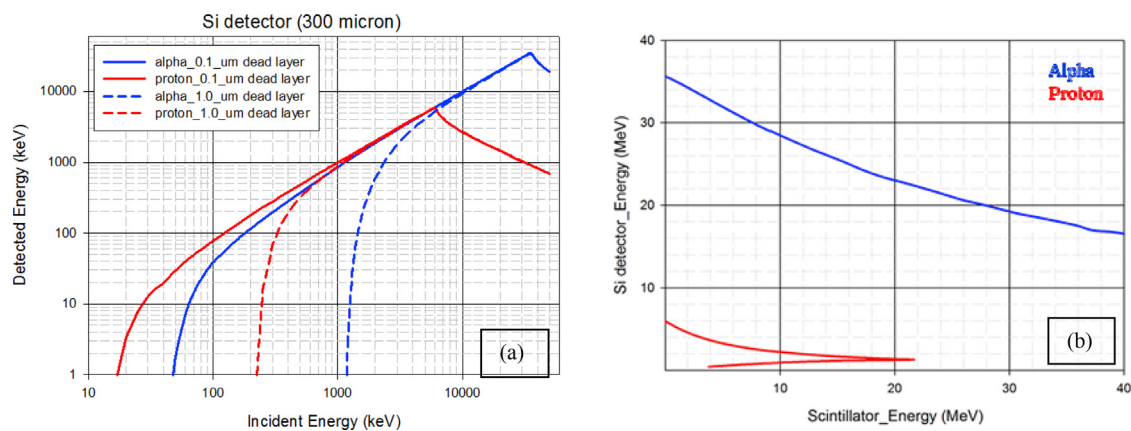
Fig. 10. (a) GEANT4 simulation for Silicon detector having two different thicknesses of entrance window, (b) GEANT4 simulation for the Energy deposited in Si detector and Scintillation detector (Agostinelli et al., 2003). (For interpretation of the references to colour in this figure legend, the reader is referred to the Web version of this article.)
