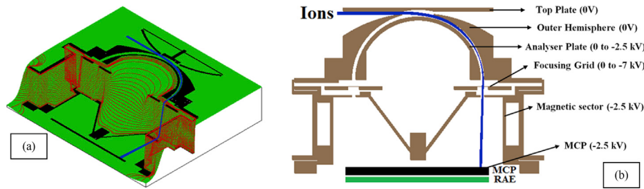
Fig. 1. (a) Potential energy view in SIMION of THA-1, (b) Various potential arrays used in the simulation with bias voltages applied to different electrodes.
