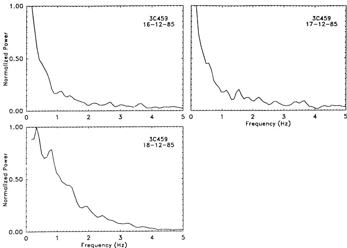
Fig. 2a-c. Shows the power spectra obtained on each day between 16 and 21 December. The spectra have been normalized to the highest spectral density and have a frequency resolution before Hanning of 0.0813 Hz. Note the clear shift in the peak of the spectrum to higher frequencies on the 18 and 19 December.
