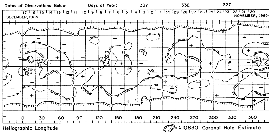
Fig. 4. H-Alpha - 10830 Å, Solar Synoptic chart showing the position of coronal holes.
