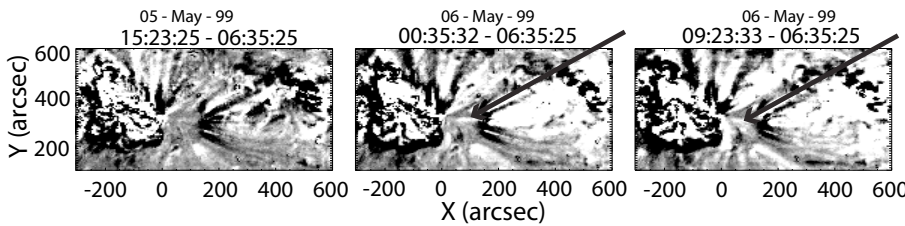
Fig. 3. Base difference images obtained at intervals of \sim 9 h. In the middle and right-hand panels, the reference image at the left at 06:35:25 UT on 05 May 1999 has been subtracted from images \sim 9 h ahead of it. The arrows in the middle and right-hand panels indicate the changes taking place in the CH.
