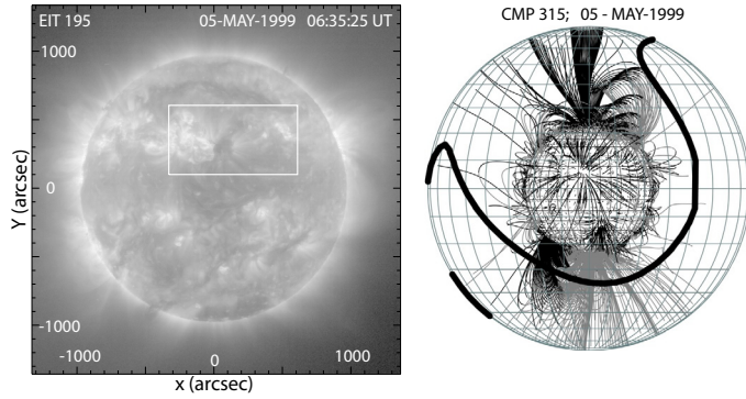
Fig. 1. Left: full-disk EIT 195 Å image on 05 May 1999. The boxed region contains AR8525 and the small CH lying against its westernmost boundary. Right: three-dimensional structure of the coronal magnetic field on 05 May 1999, with the field lines projected on to a source surface at 2.5 R_{\odot} . The thick wavy line is the magnetic neutral line. See text for details.
