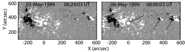
Fig. 4. MDI magnetograms of the boxed region of the solar disk from Fig. 1. The panels differ in time by a little over 24 h. Arrow 1 shows a small region of newly emerging negative flux while arrows 2 and 3 show two evolving bipolar regions.
