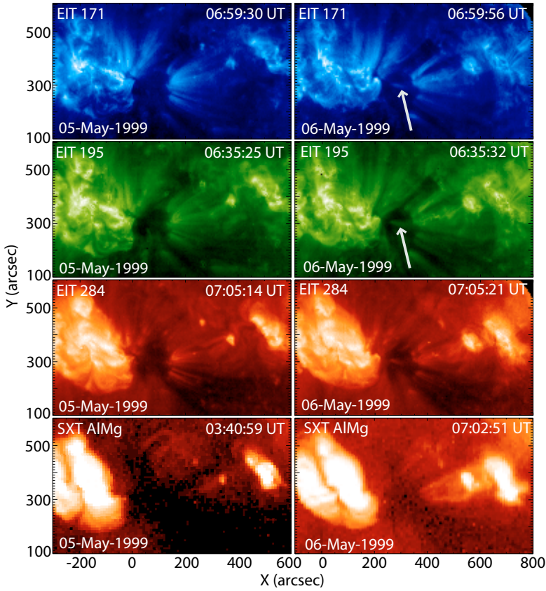
Fig. 2. The boxed region of the solar disk from Fig. 1 on 05 May 1999 (left column) and 06 May 1999 (right column). From the top down are shown respectively, EIT 171 Å; EIT 195 Å; 284 Å; and an SXT image. The white arrows in two of the right-hand panels point to new bright features in the CH.
