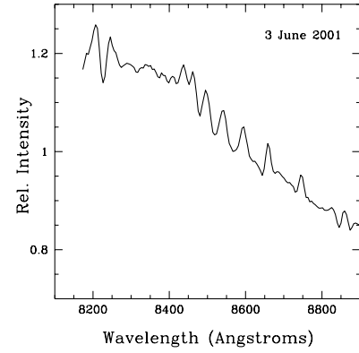
Fig. 2. The Paschen 11–20 emission lines in \delta Sco. The H 2 O band absorption head at 8227 Å can be seen.
