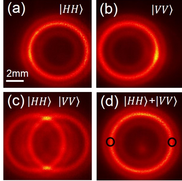
Figure 3.3.5: Images of the paired photons of polarization state, (a) |HH\rangle , (b) |VV\rangle , (c) both |HH\rangle and |VV\rangle with misalignment, and (d) perfectly overlapped states, |HH\rangle and |VV\rangle . The black circles represent the diametrically opposite regions on the SPDC ring used for entanglement studies. The pump power used for this measurement is 5 mW.
