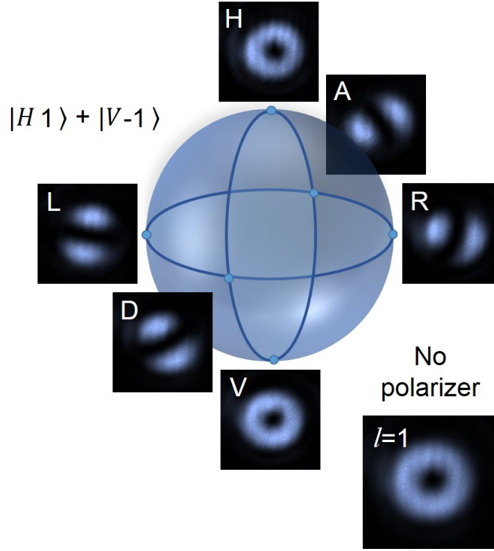
Figure 6.4.2: Intensity profiles of the non-separable states of the pump beam for two different OAM modes. Depending on the projection of the beam in different polarization states, |H\rangle , |A\rangle , |R\rangle , |V\rangle , |D\rangle , and |L\rangle (as shown by the white letters on the images) on the Poincaré sphere, the mode pattern of the beam recorded by the CCD camera changes to different points on LG-Bloch sphere for state \frac{1}{\sqrt{2}}(|H1\rangle + e^{-i\phi}|V-1\rangle) .
