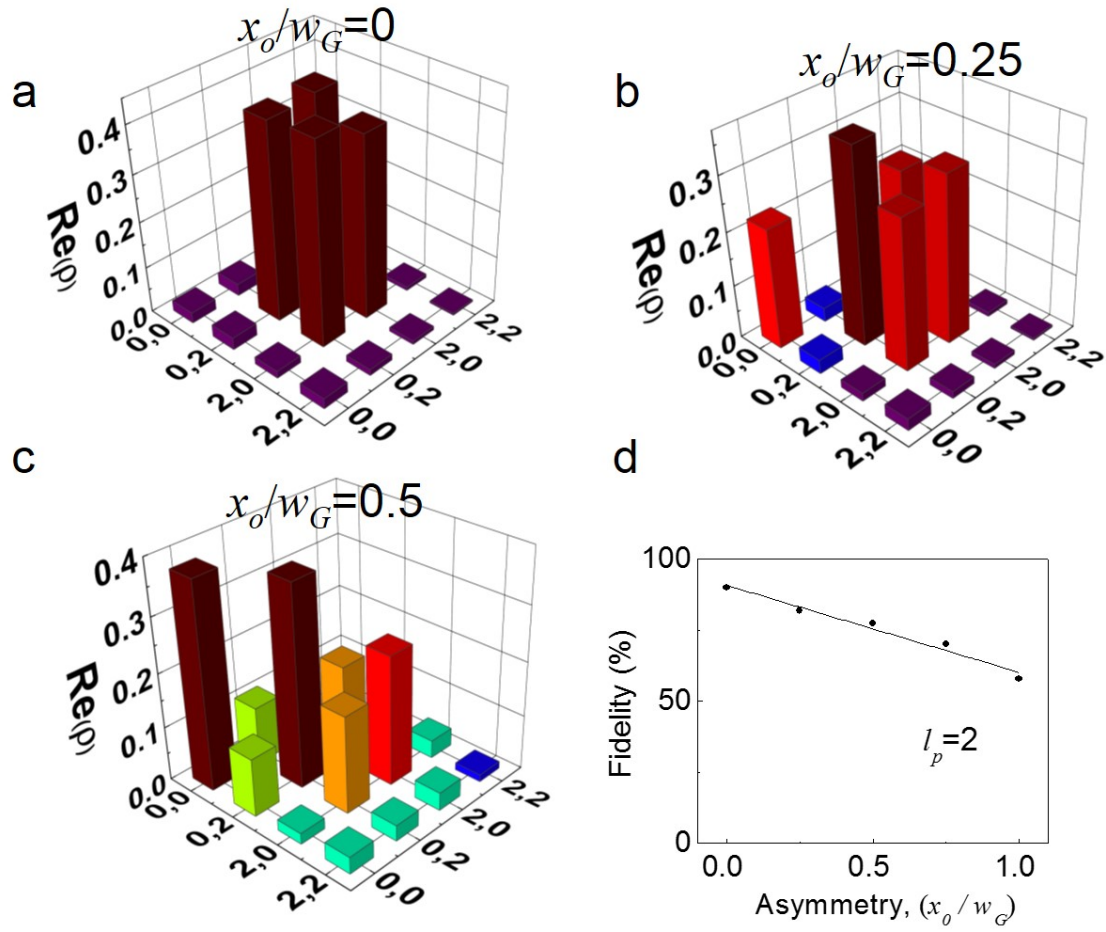
Figure 7.3.5: (a-c) Variation of the density matrix of two dimensional OAM entangled state with the asymmetry, x_o/w_G=0, 0.25 and 0.5 of pump vortex OAM mode, l_p=2 . (d), The change in the fidelity of the state with pump beam asymmetry.
