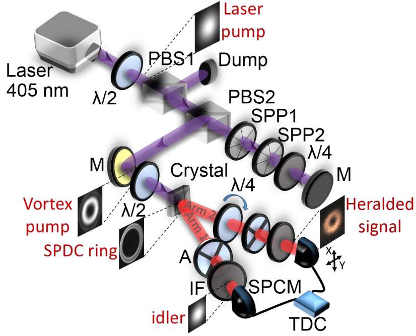
Figure 5.2.1: Schematic of the experimental setup. \lambda/2 , half-wave plate; PBS1-2, polarizing beam splitter cube; SPP1-2, spiral phase plates; \lambda/4 , quarter-wave plate; M1-2, Mirrors; Crystal, dual-BiBO for generation of entangled photons; IF, interference filter; SPCM, single photon counting module; TDC, time to digital converter; 2D images show the spatial profile at the respective point.
