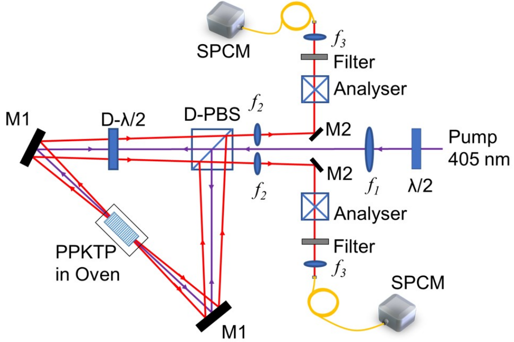
Figure 3.2.1: Schematic of the experimental setup. \lambda/2 , half-wave plate at 405 nm; D-PBS, D- \lambda/2 , polarizing beam splitter cube and half-wave plate at dual wavelengths, at 405 nm and 810 nm; M1-2, mirrors; f_{1-3} , lenses; PPKTP, nonlinear crystal in a temperature oven; Analyzer, polarization analyzer comprises a PBS and a \lambda/2 plate; IF, interference filter; SPCM, single photon counting module.
