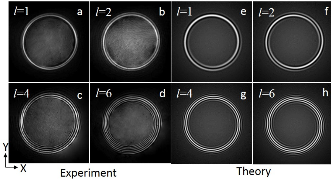
Figure 4.4.2: (a-d) Experimentally measured interference pattern and (e-h) corresponding theoretical interference pattern of the perfect vortex of order l=1, 2, 4 and 6 and Gaussian beam.
