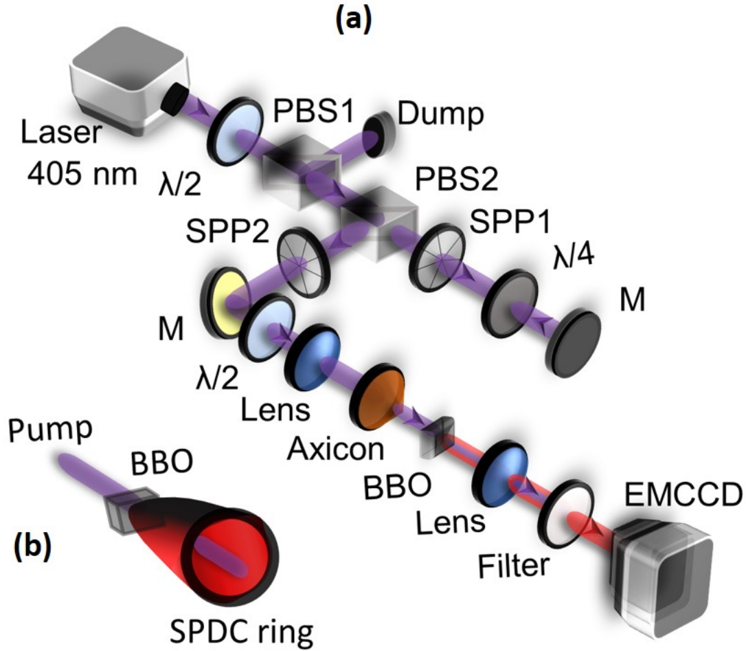
Figure 4.3.1: (a) Schematic of the experimental setup. \lambda/2 , half wave plate; PBS1-2, polarizing beam splitter cube; SPP1-2, spiral phase plate; \lambda/4 , quarter wave plate; M1-2, Mirrors; Axicon, to generate BG beam; BBO, nonlinear crystal for down conversion; Filter, interference filter; EMCCD, electron multiplying CCD. (b) Schematic of generation of SPDC ring.
