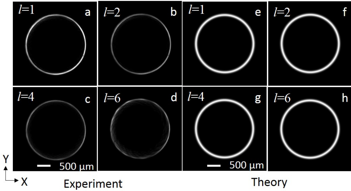
Figure 4.4.1: (a-d) Experimentally measured intensity distribution and (e-h) corresponding theoretical intensity distribution of the perfect vortex of order l=1, 2, 4 and 6 .
