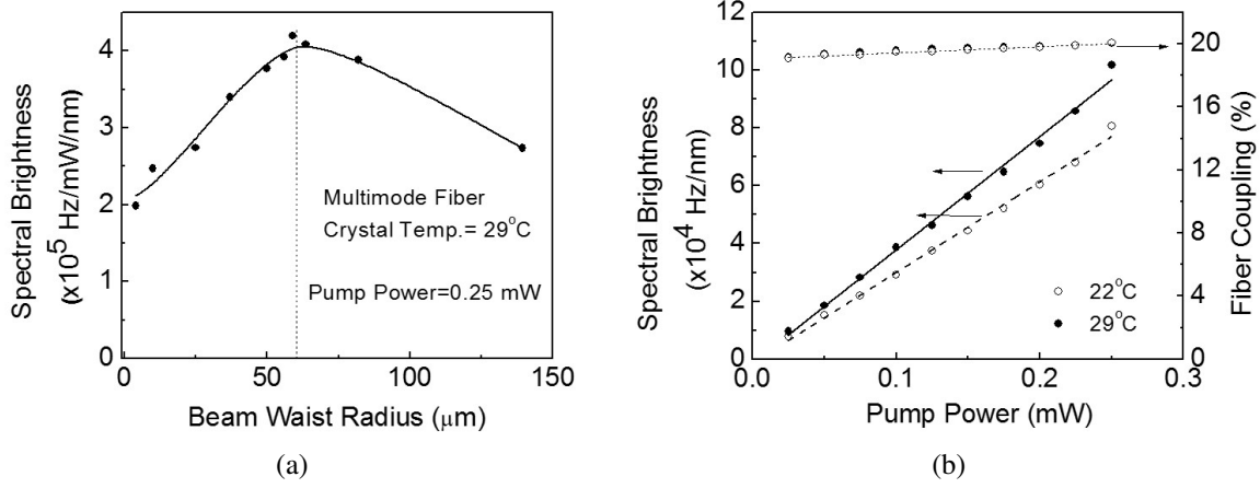
Figure 3.3.3: (a) Dependence of spectral brightness of the paired photons on the pump beam waist at crystal temperature of 29° C, and (b) the variation of spectral brightness and fiber coupling efficiency on the pump power at crystal temperature 22° C (open circles) and 29° C (solid circles) for photon collection using multimode fiber.
