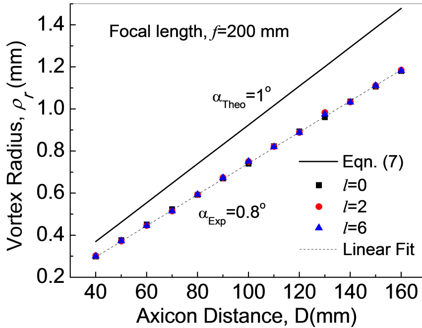
Figure 4.4.4: Variation of perfect vortex radius with distance D for vortex order 0, 2 and 6. The solid points and dotted line represent the experimental data and linear fit, respectively. Solid line represents theoretical beam radius of the perfect vortex calculated using Eq. (7) and axicon parameters.
