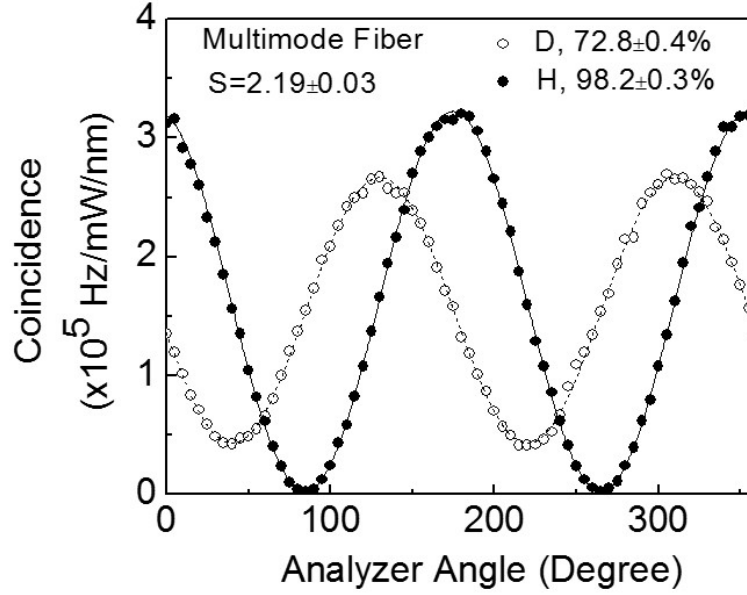
Figure 3.3.6: Quantum interference of the entangled photons at horizontal, H (solid circles) and diagonal, D (open circles) projection bases for crystal temperature 29^\circ \text{C} collected using multimode fiber
