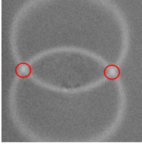
Figure 2.2.2: Intensity profile of the down converted photons generated under non-collinear type-II phase-matching condition.
