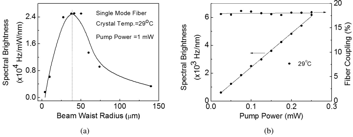
Figure 3.3.4: (a) Dependence of spectral brightness of the paired photons on the pump beam waist, and (b) the variation of spectral brightness and fiber coupling efficiency with the pump power at crystal temperature of 29° C for photon collection using singlemode fiber. Lines are guide to the eye.
