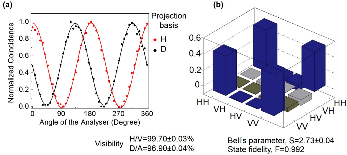
Figure 6.4.1: (a) Visibility graph for polarization entangled state at H (red dots) and D (black dots) bases. (b) Graphical representation of the density matrix obtained from linear tomographic technique for polarization entangled state.
