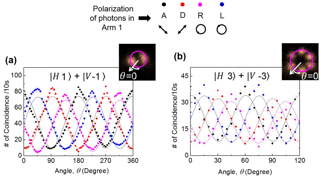
Figure 6.4.6: (a) Coincidence per angular region for A (black dots), D (red dots), R (pink dots) and L (blue dots) projections of the idler photon for OAM l=1 , (b) for l=3 . The lines are theoretical fit to experimental data. (Inset) Image of the probability distribution of the heralded signal photons. Errors are estimated from iteration.
