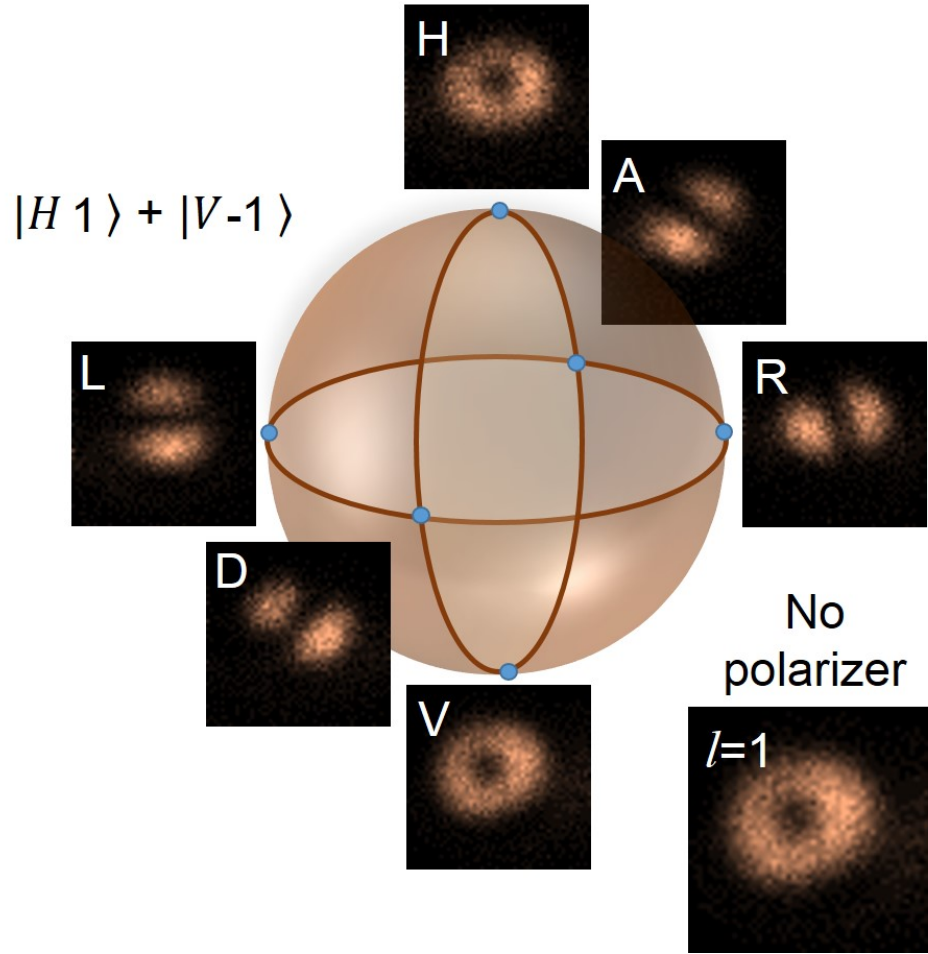
Figure 6.4.4: Gallery of images representing the probability distribution of the heralded signal photons. Depending on the polarization of the idler photon projected (white letters in the images) at different points in the polarization Poincaré sphere, the spatial distribution of the heralded signal changes into different mode patterns in the LG-Bloch sphere. The sequence of coincidence images of the heralded signal due to particular polarization of its partner (idler) photon while pumping with non-separable states of first order ( l = 1 ) LG modes around the meridian (vertical circle) and the equator (horizontal circle) in the LG-Bloch sphere confirms the generation of hybrid entangled two photon states encoded in polarization and OAM. In absence of any polarizer in the path of the idler photon, the spatial distribution of the heralded signal photon (inset) shows a statistical mixture of all states of the LG-Bloch sphere.
