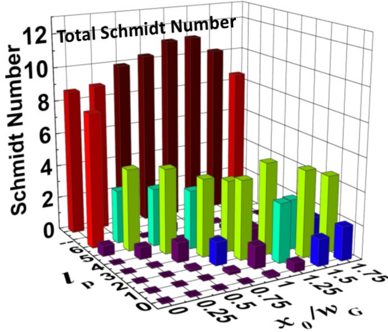
Figure 7.3.4: Variation in the measured value of Schmidt number, K , as a function of asymmetry in the pump vortex beam.
