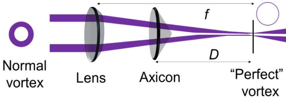
Figure 4.2.1: Pictorial representation of the generation of variable size perfect vortex by using lens-axicon combination.
