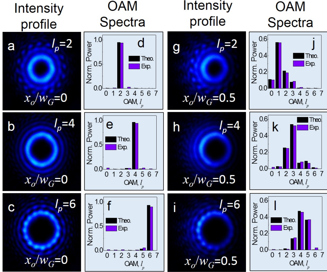
Figure 7.3.1: (a-c) Far-field intensity distribution of symmetric vortex beam ( x_o/w_G=0 ) and (d-f) corresponding OAM spectra, (g-i) intensity distribution of the asymmetric ( x_o/w_G=0.5 ) pump vortex beams and (j-l) corresponding OAM spectra, of orders, l_p= 2, 4 , and 6 . The black and violet bars represent the theoretical and experimental results respectively..
