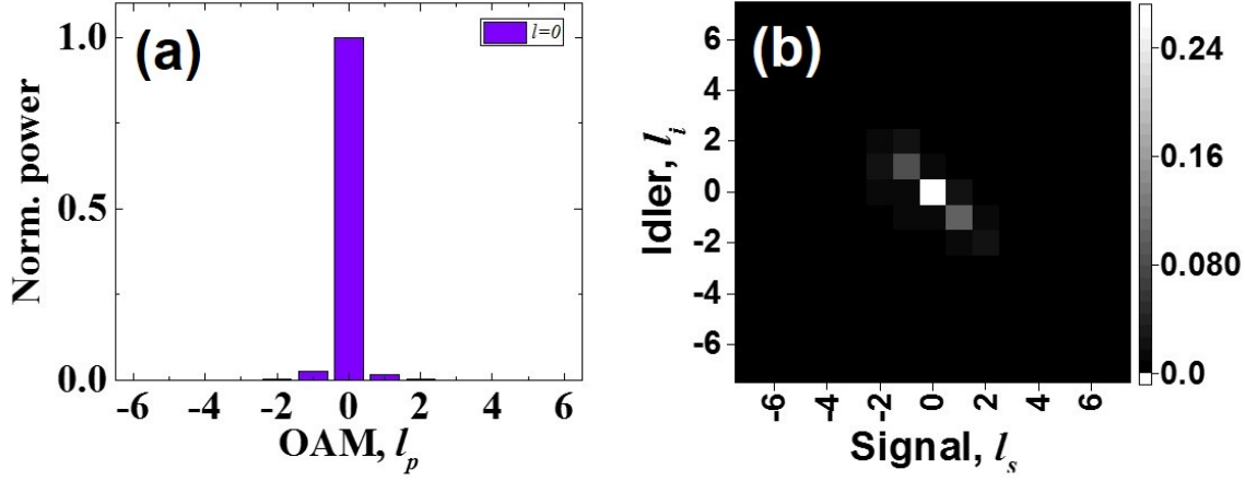
Figure 7.3.2: (a) OAM spectrum of pump Gaussian and (b) measured bi-photon eigen OAM modes in SPDC process.
