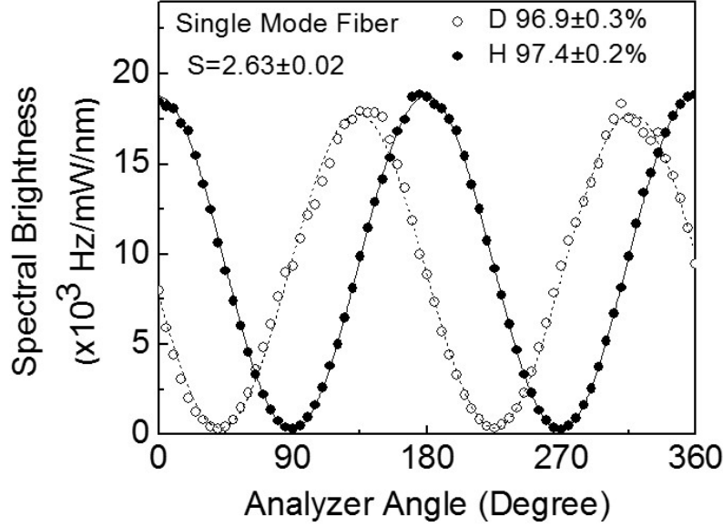
Figure 3.3.7: Quantum interference of the entangled photons at horizontal, H (solid circles) and diagonal, D (open circles) projection bases for crystal temperature 29° C collected using single mode fiber
