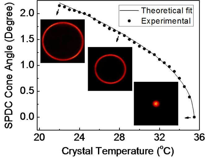
Figure 3.3.1: Variation of emission half-cone angle of the SPDC photons measured in free space with crystal temperature. Solid line corresponds to the theoretical fit to the experimental data. (Inset) CCD images of the SPDC ring at three crystal temperatures, 22°C, 28°C and 35°C
