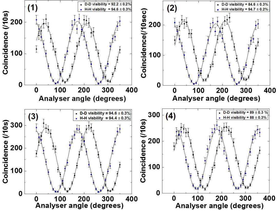
Figure 5.3.3: Variation in coincidence counts when the analyzer at the arm 2 rotates and the analyzer at arm 1 is kept at 45^\circ (black dots) for D-D projection and at 0^\circ (blue dots) for H-H projection at point (1)-(4) while pumped with vortex beam.
