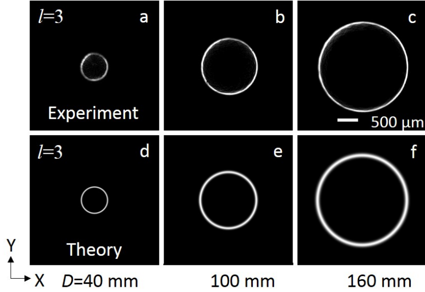
Figure 4.4.3: Experimental and theoretical images of the perfect vortex of order l=3 for different positions of the axicon. First row and second row respectively represent the experimental and theoretical images of the perfect vortex for D value (a,d) 40 mm, (b,e) 100 mm, (c,f) 160 mm.
