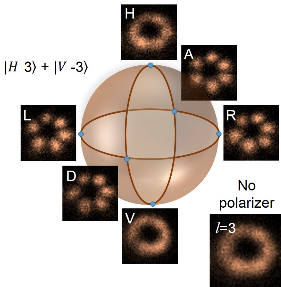
Figure 6.4.5: Gallery of images representing the probability distribution of the heralded signal photons. Depending on the polarization of the idler photon projected (white letters in the images) at different points in the polarization Poincaré sphere, the spatial distribution of the heralded signal change into different mode patterns in the LG-Bloch sphere. The sequence of coincidence images of the heralded signal due to particular polarization of its partner (idler) photon while pumping with non-separable states of third order ( l = 3 ) LG modes around the meridian (vertical circle) and the equator (horizontal circle) in the LG-Bloch sphere confirms the generation of hybrid entangled two photon states encoded in polarization and OAM. In absence of any polarizer in the path of the idler photon, the spatial distribution of the heralded signal photon (inset) shows a statistical mixture of all states of the LG-Bloch sphere.
