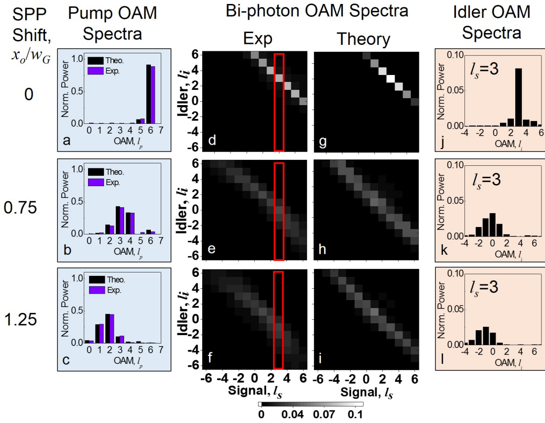
Figure 7.3.3: (a-c) Distribution of OAM modes of asymmetric pump beam of x_o/w_G=0, 0.75 and 1.25 , corresponding spiral spectrum for bi-photon OAM eigenmodes (d-f), measured and (g-i) simulated. (j-l) A portion of the spiral spectrum of idler at a fixed OAM mode ( l_s=3 ) of the signal.
