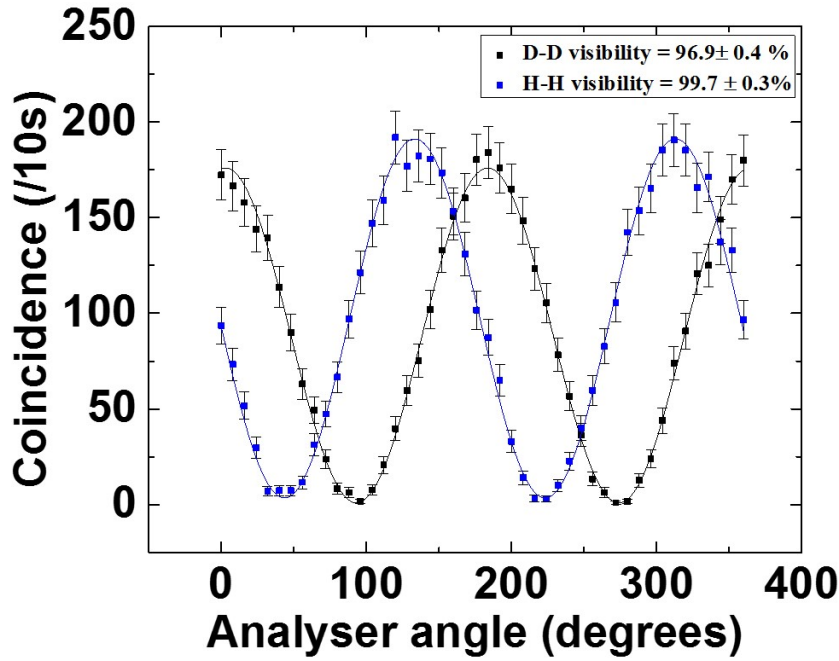
Figure 5.3.1: Variation in coincidence counts when the analyzer at the idler arm rotates while the analyzer at signal arm is kept @ 45^\circ (black dots) for D-D projection and @ 0^\circ (blue dots) for H-H projection while pumped with Gaussian beam.
