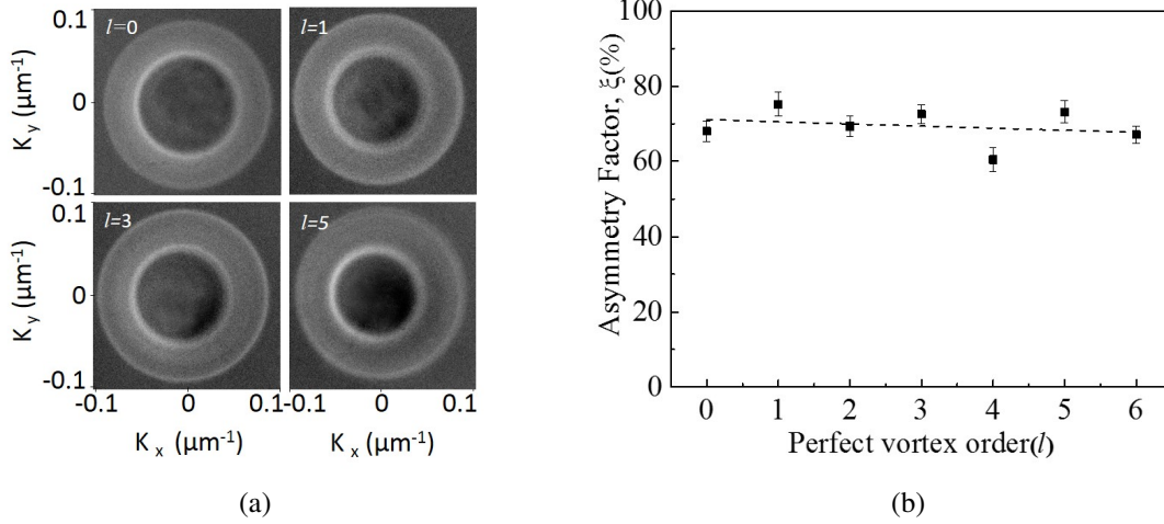
Figure 4.4.7: (a) Angular spectrum (transverse momentum) of the down converted photons recorded using EMCCD with perfect vortex radius \rho_r = 1.18 mm for topological charge l = 0, 1, 3 , and 5. K_x and K_y are the transverse momentum components. (b) Dependence of asymmetry of the angular spectrum of the down converted photons on OAM of the pump vortex beam.
