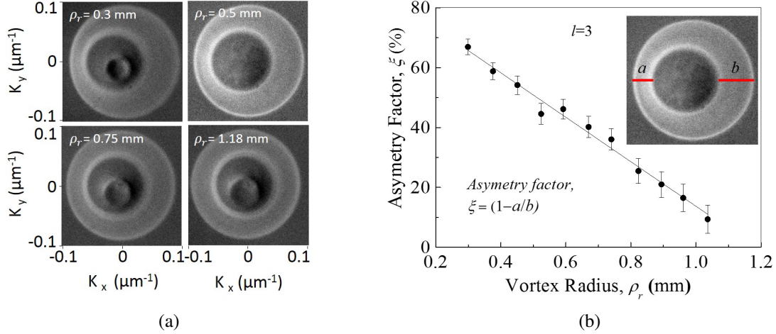
Figure 4.4.6: (a) Angular spectrum (transverse momentum) of the down converted photons recorded using EMCCD with vortex order l=3 for pump beam radius of, 0.3, 0.5, 0.75, and 1.18 mm. K_x and K_y are the transverse momentum components. (b) Dependence of asymmetry of the angular spectrum of the down converted photons on the radius of pump vortex beam. Asymmetry parameter is defined as \xi = (1-a/b) , where, 'a' and 'b' are quantified as the separation between two rings on left and right side of the transverse momentum distribution of the down converted photons (inset).
