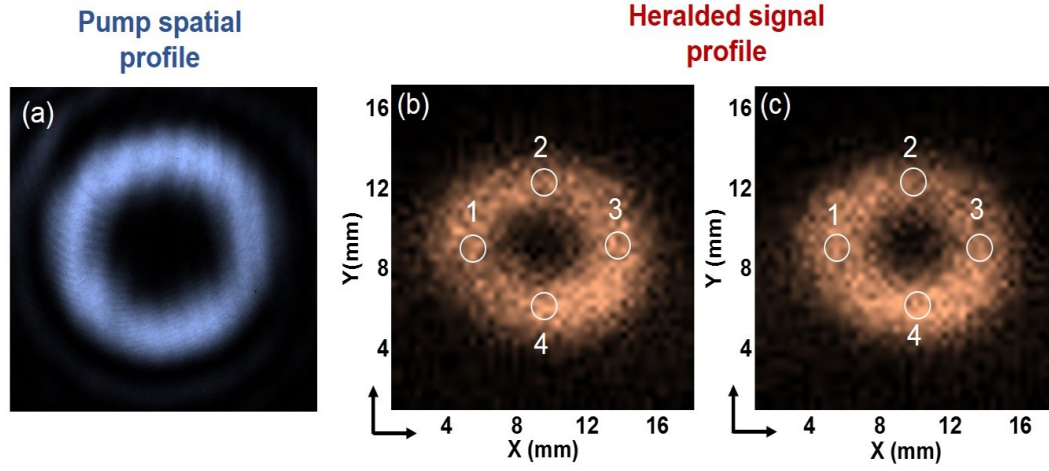
Figure 5.3.2: (a) Intensity profile of the pump vortex beam. (b) Horizontal and (c) Vertical polarized heralded signal photons generated from each crystals independently.
