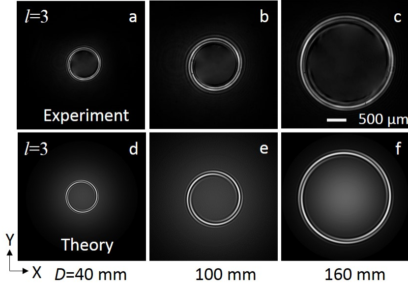
Figure 4.4.5: (a-c) Experimentally measured interference pattern and (e-f) corresponding theoretical interference pattern of the variable perfect vortex of order l=3 generated at different D=40, 100 and 160 mm with Gaussian beam.
