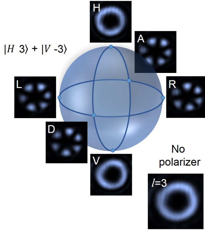
Figure 6.4.3: Intensity profiles of the non-separable states of the pump beam for two different OAM modes. Depending on the projection of the beam in different polarization states, |H\rangle , |A\rangle , |R\rangle , |V\rangle , |D\rangle , and |L\rangle (as shown by the white letters on the images) on the Poincaré sphere, the mode pattern of the beam recorded by the CCD camera change to different points on LG-Bloch sphere for the state \frac{1}{\sqrt{2}}(|H3\rangle + e^{-i\phi}|V-3\rangle) .
