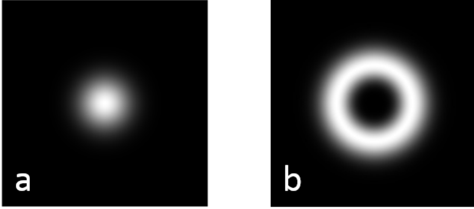
Figure 2.3.1: Intensity profile of (a) Gaussian beam and (b) Vortex beam.
