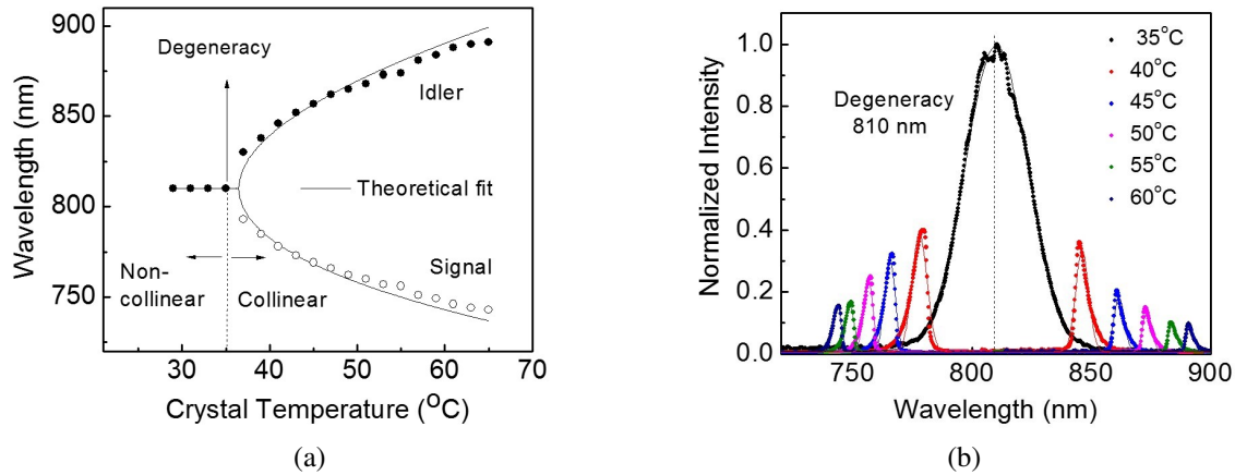
Figure 3.3.2: (a) Wavelength tuning of the SPDC photons as a function of crystal temperature. (b) Emission spectra of the SPDC photons recorded at different crystal temperatures.
