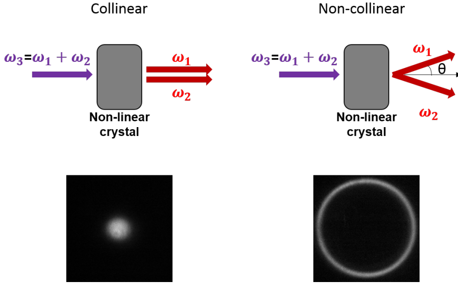
Figure 2.2.1: First row shows the pictorial representation of collinear and non-collinear phase-matching and the second row shows the intensity profile of the down converted photons generated in the respective configuration.
