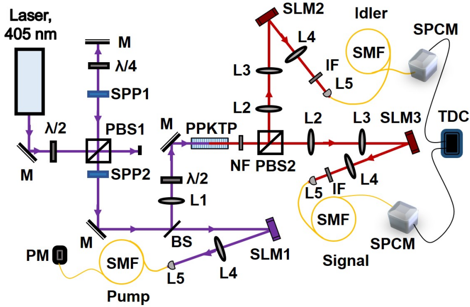
Figure 7.2.1: Schematic of the experimental setup. \lambda/2 , \lambda/4 , half-wave plate and quarter wave plate at 405 nm, respectively; PBS, polarizing beam splitter cube at 405 nm and 810 nm respectively; SPP1-2, spiral phase plate; M, mirrors; L1-5, lenses; PPKTP, non-linear crystal in a temperature oven; SLM, spatial light modulator; IF, interference filter; NF, notch filter; SMF, single mode fibre; SPCM, single photon counting module; TDC, coincidence counter; PM, power meter
