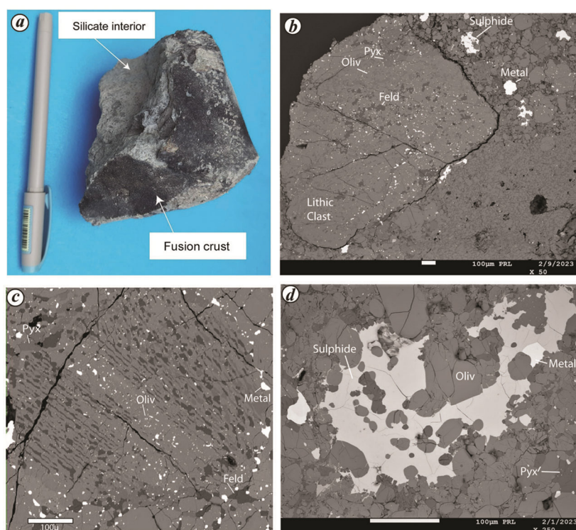
Figure 2. a , Hand specimen of Kopergaon meteorite. Black fusion crust and grey silicate interior are shown. Length of the pen is 14 cm. b , c , Back-scattered electron (BSE) images of Kopergaon fragmental breccia. Lithic clasts and chondrule clasts are shown. Oliv, Olivine; Feld, Feldspar; Pyx, Pyroxene. d , BSE image of sulphide (troilite) and metal (Fe-Ni alloy) in Kopergaon chondrite.
